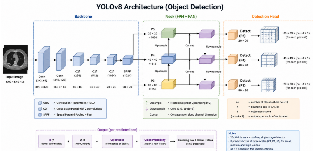
Figure 3.17: Detailed architectural diagram of the YOLOv8 object detection framework, illustrating the Backbone, Neck (FPN + PAN), and Detection Head stages for multi-scale prediction.
