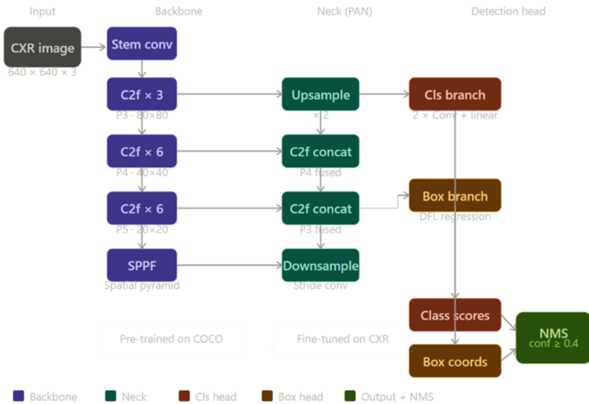
Figure 3.13: YOLOv8 architecture pipeline for automated localization and classification of pulmonary abnormalities.
