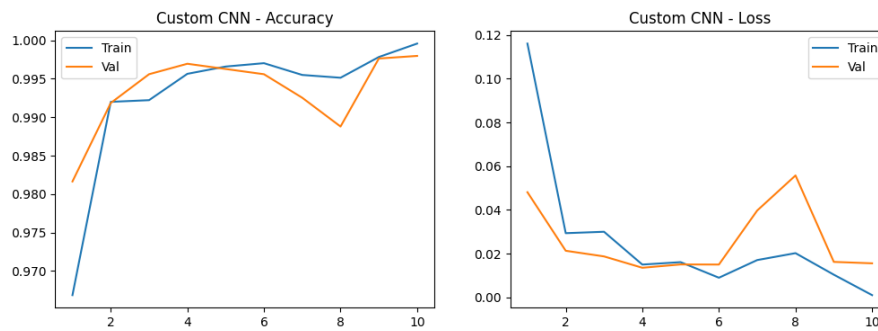
(a) Training and validation curves for the Custom CNN model.
