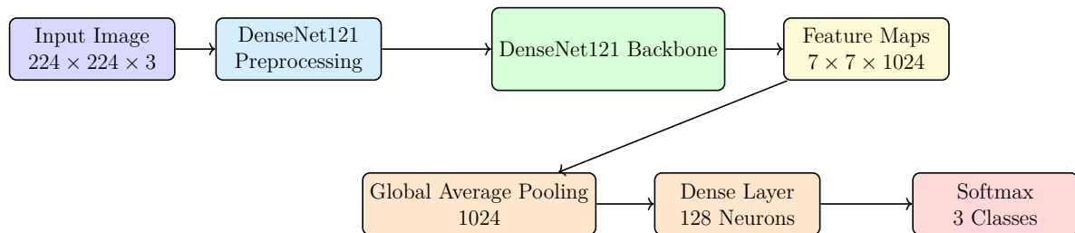
Figure 3.6: Two-row architecture of the DenseNet121-based medical image routing model.
