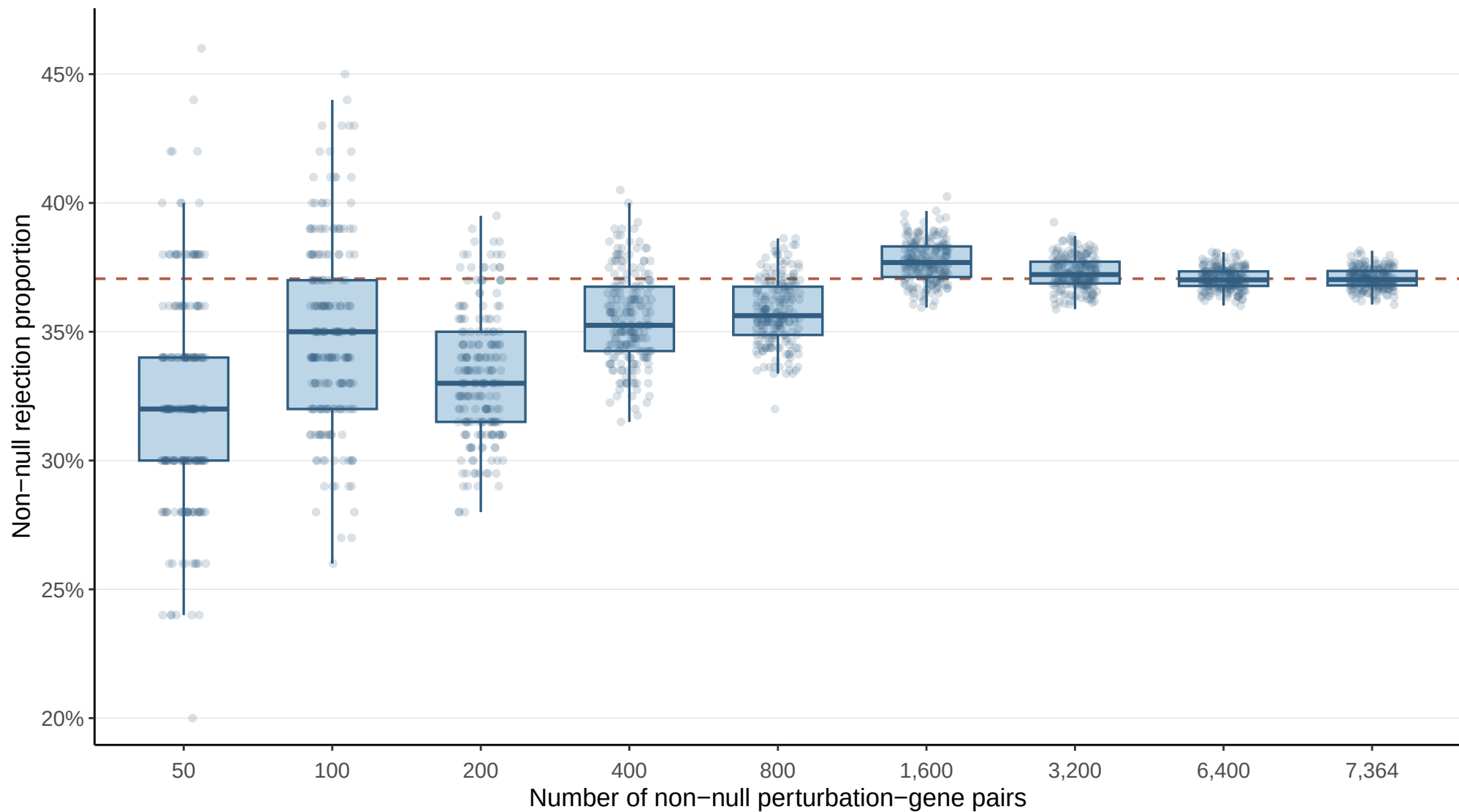
SCEPTRE power across simulated runs: num_trt_1250
