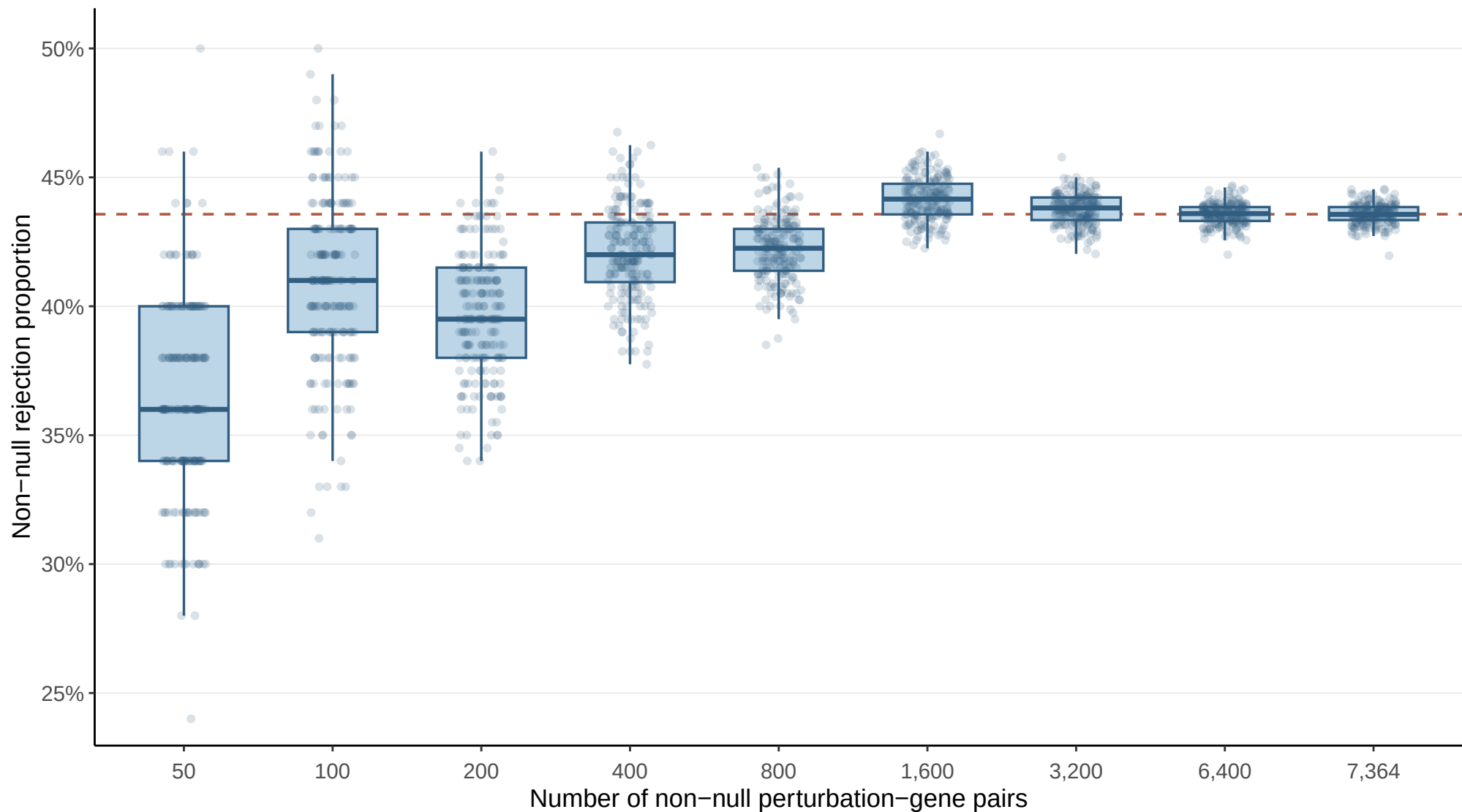
SCEPTRE power across simulated runs: num_trt_1750
