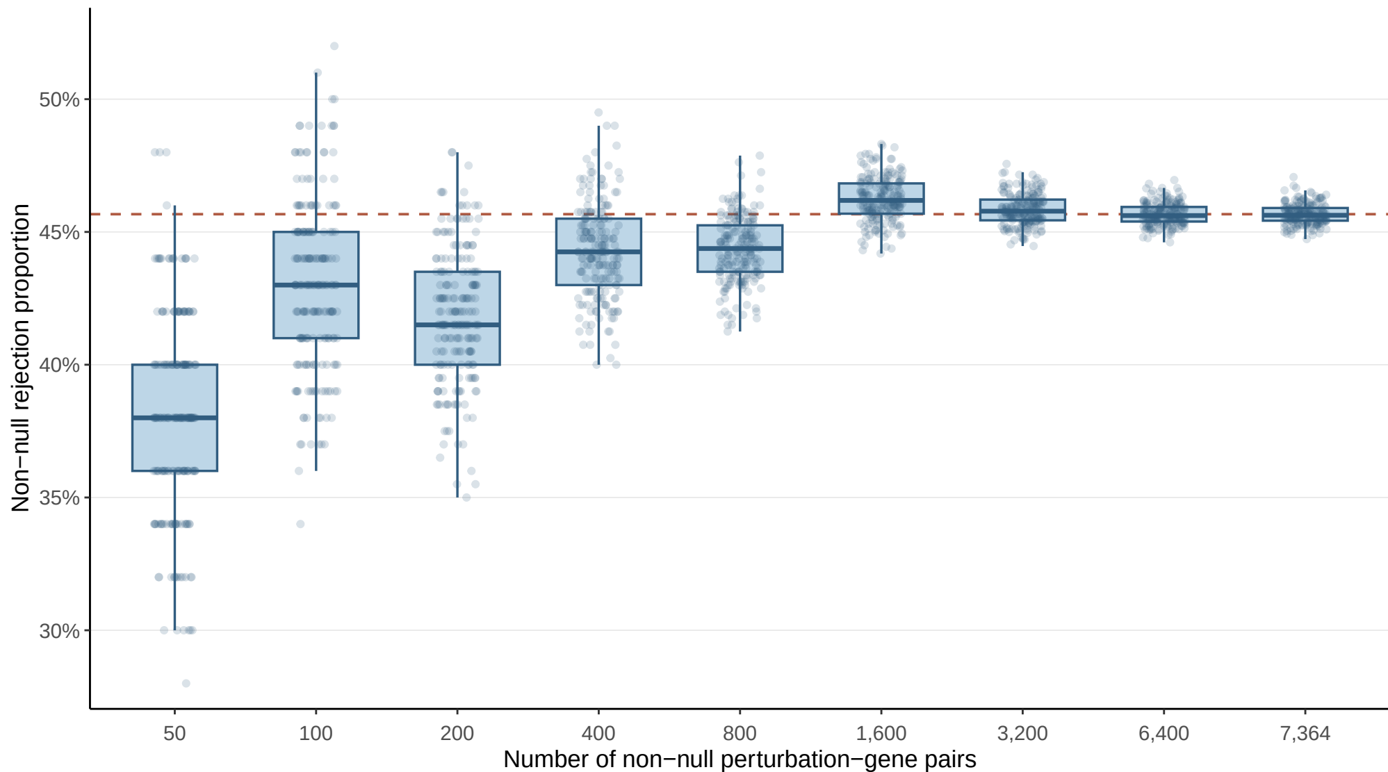
SCEPTRE power across simulated runs: num_trt_2000
