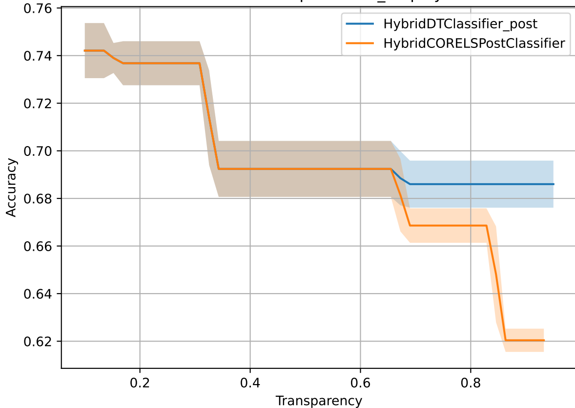
Validation-Depth: 1-acs_employ
