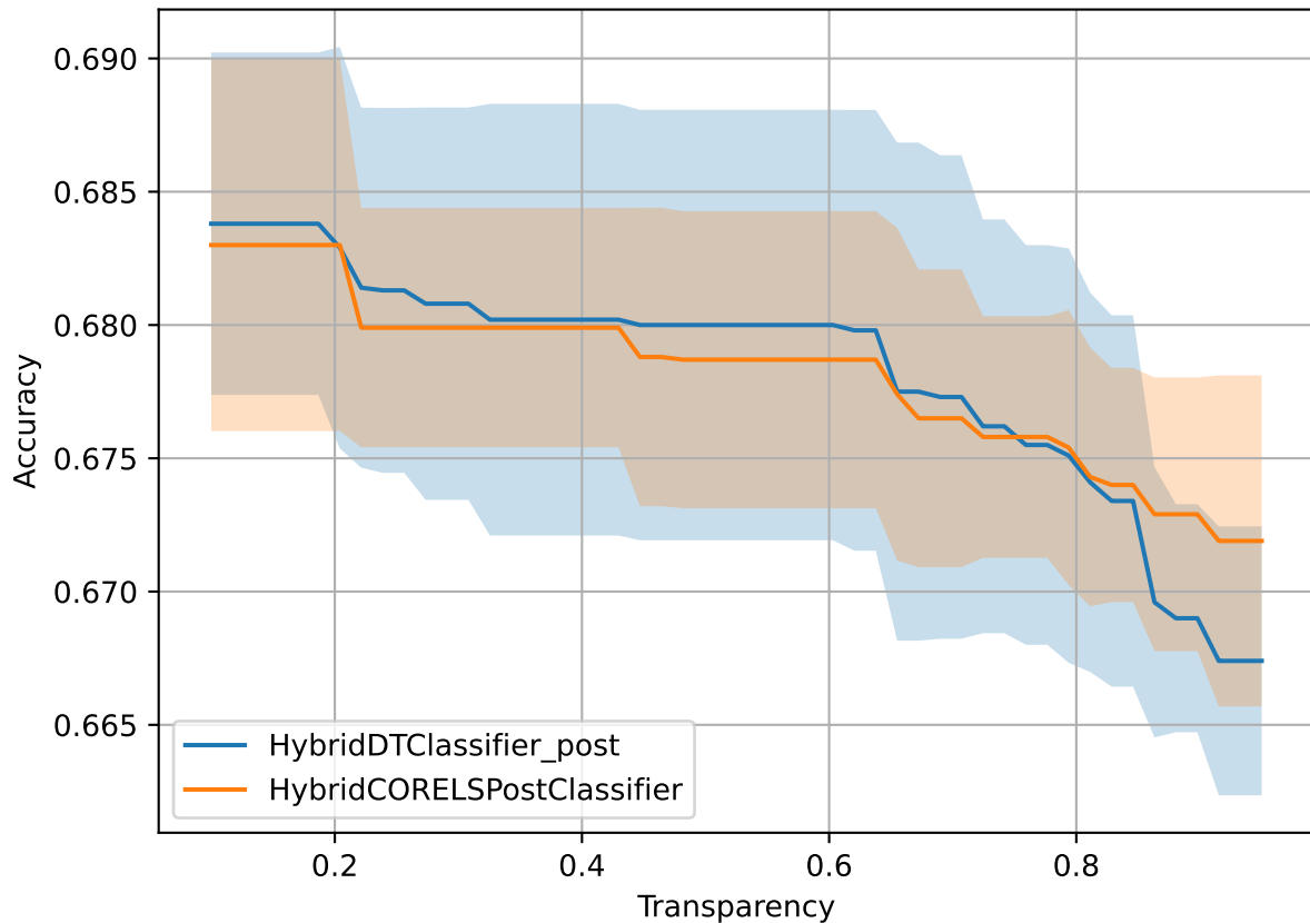
Validation-Depth: 5-compas
