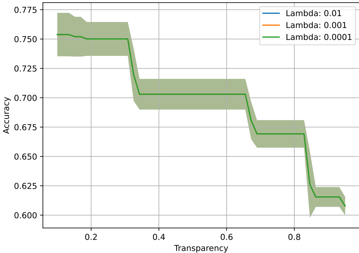
Train-Depth: 1-acs_employ
