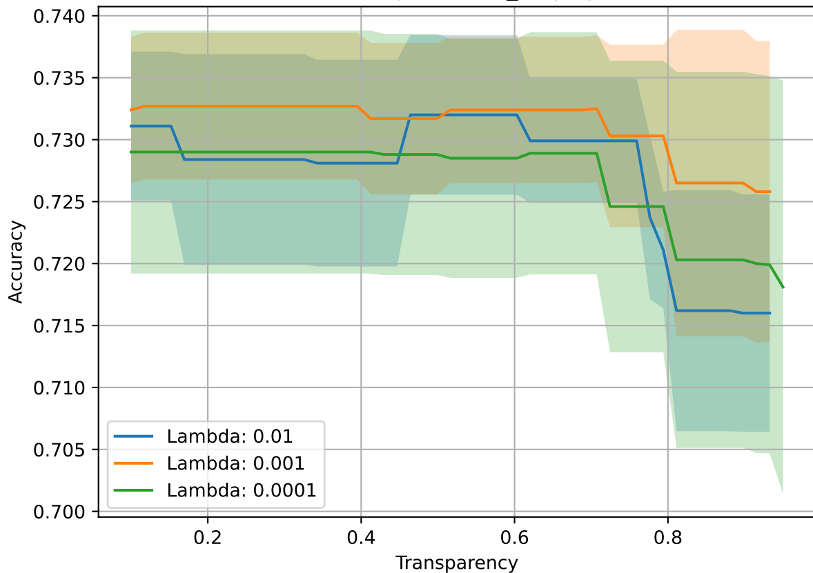
Test-Depth: 4-accs_employ
