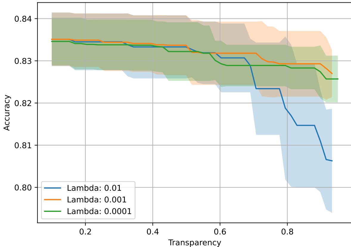
Validation-Depth: 4-adult
