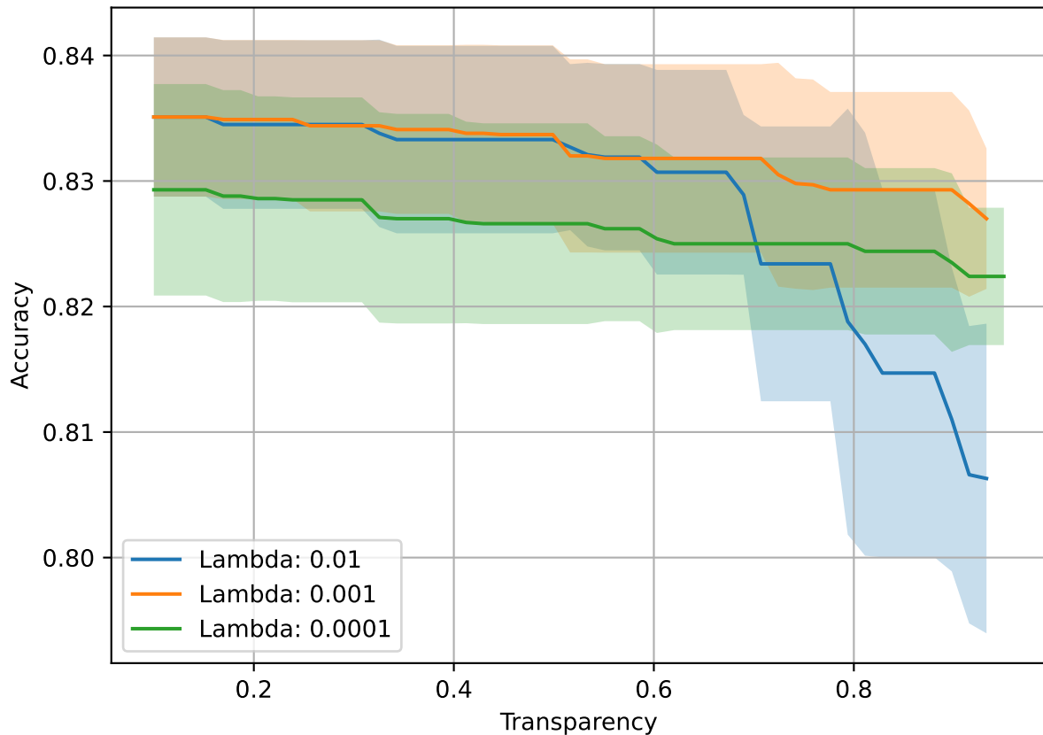
Validation-Depth: 5-adult
