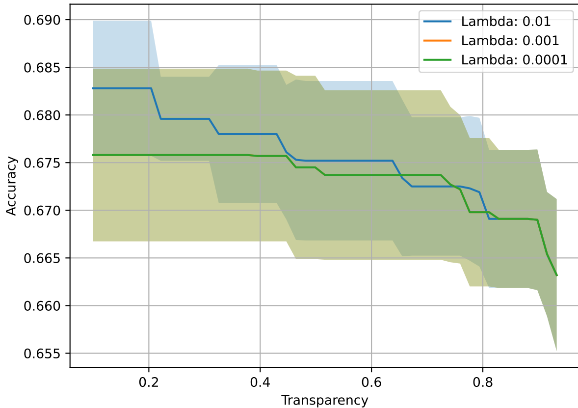
Validation-Depth: 2-compas
