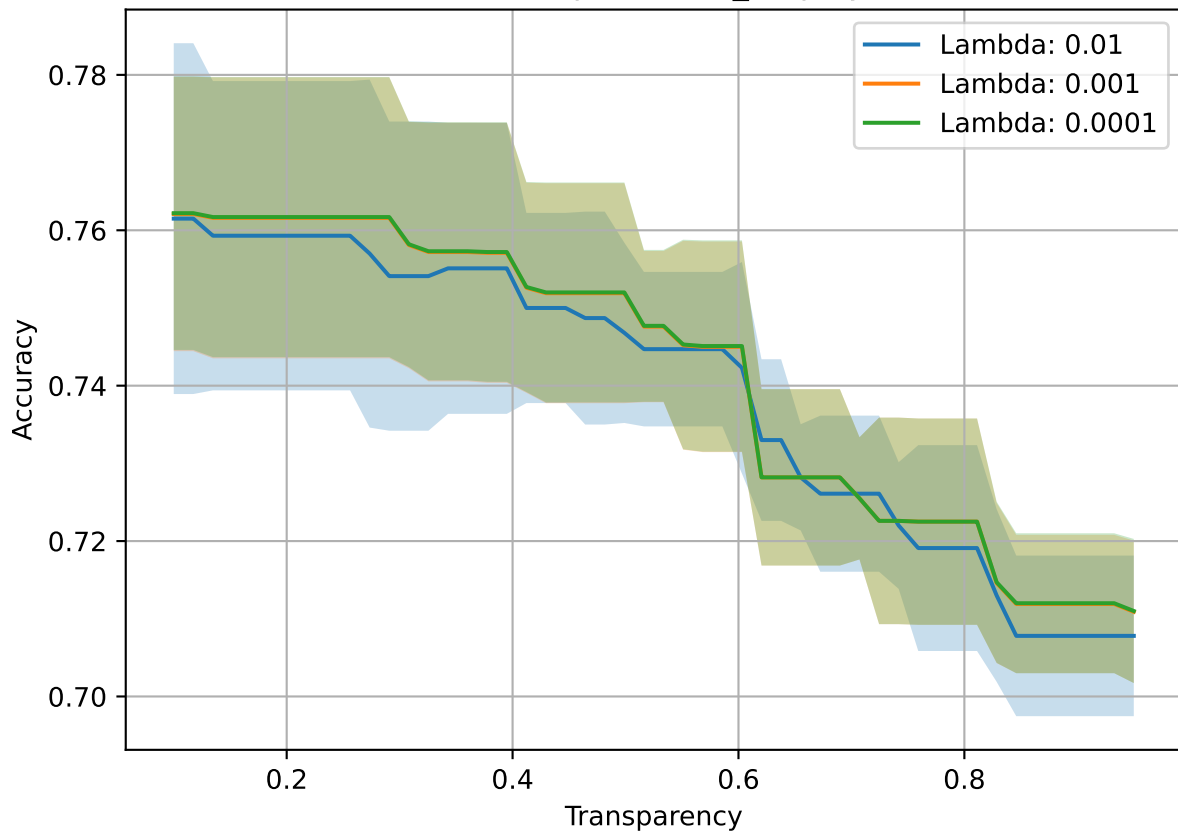
Train-Depth: 2-acs_employ
