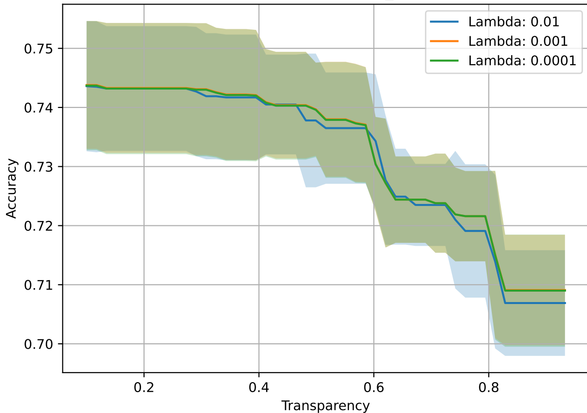
Validation-Depth: 2-acs_employ
