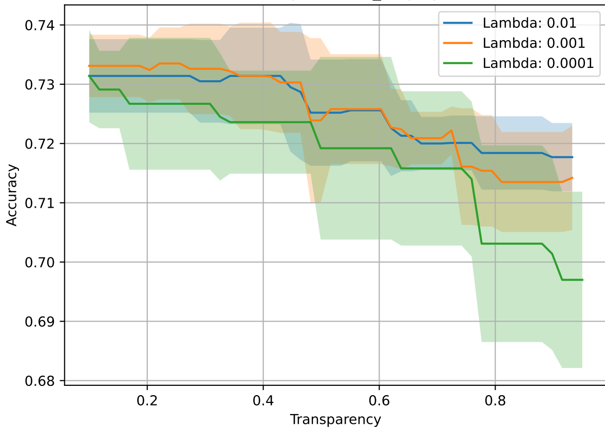
Test-Depth: 3-acs_employ
