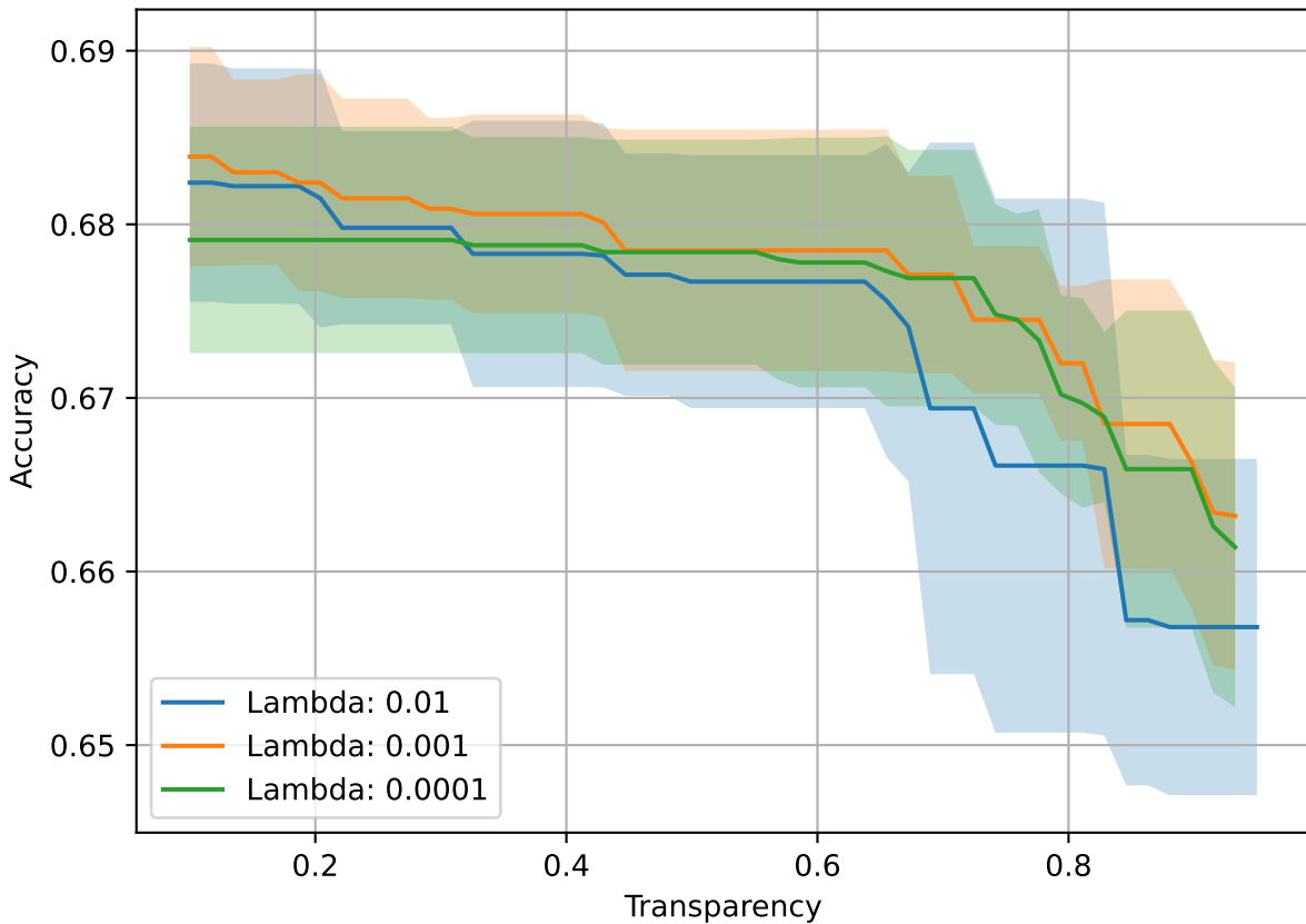
Validation-Depth: 4-compas
