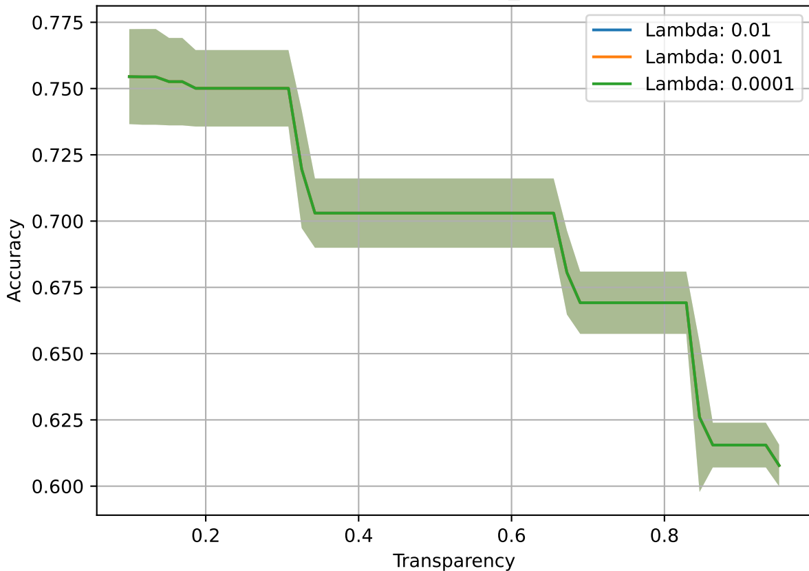
Train-Depth: 1-acs_employ
