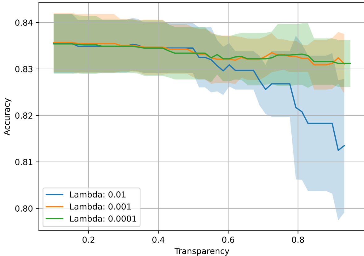
Test-Depth: 4-adult
