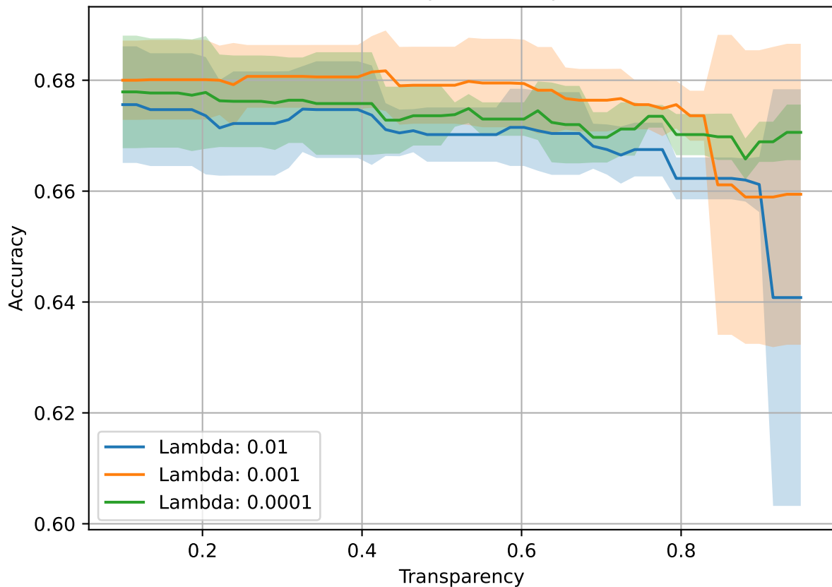
Train-Depth: 5-compas
