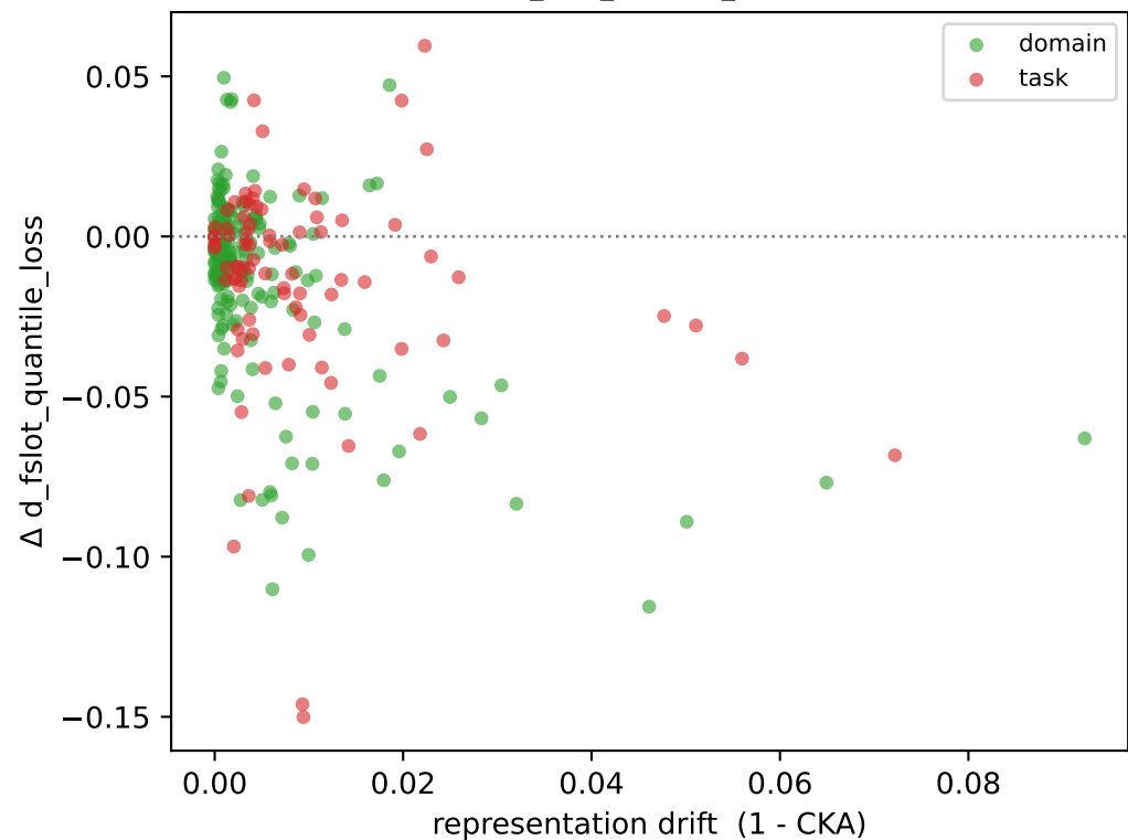
d_fslot_quantile_loss
