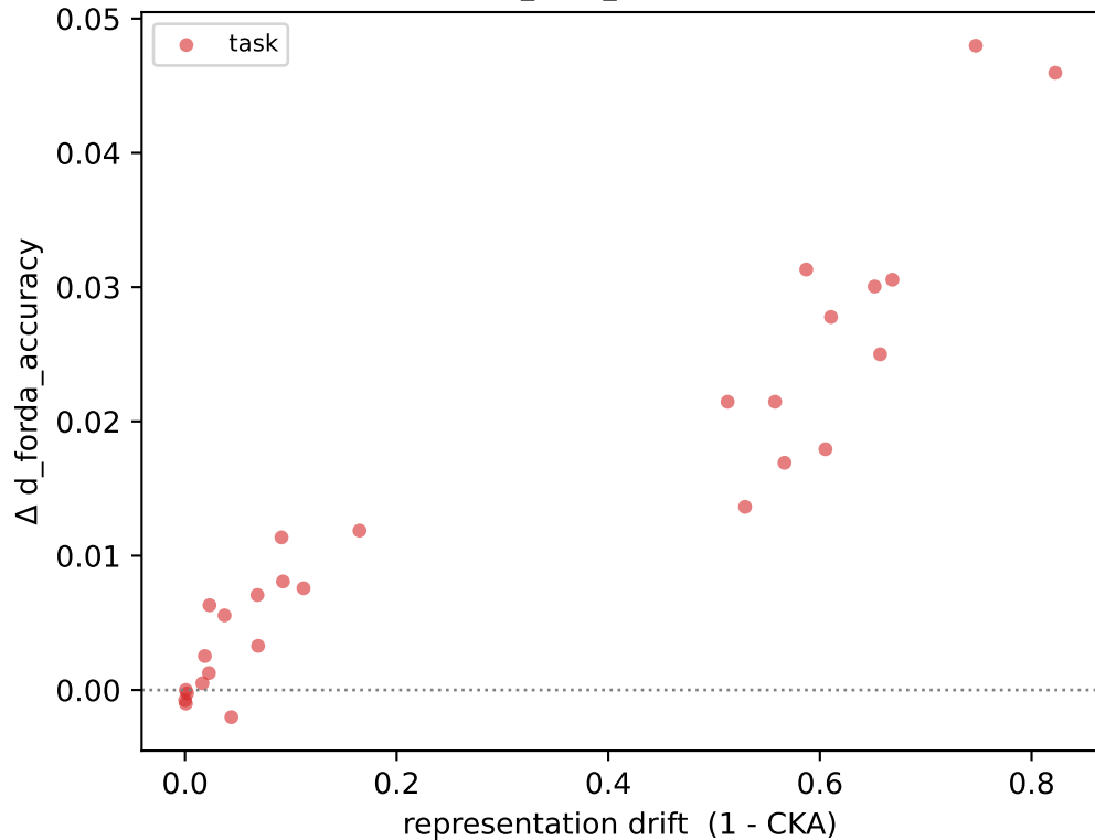
d_forda_accuracy
