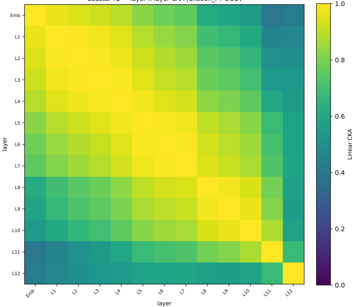
Coastal-TS — layer x layer CKA (unseen_PT-OOD)
