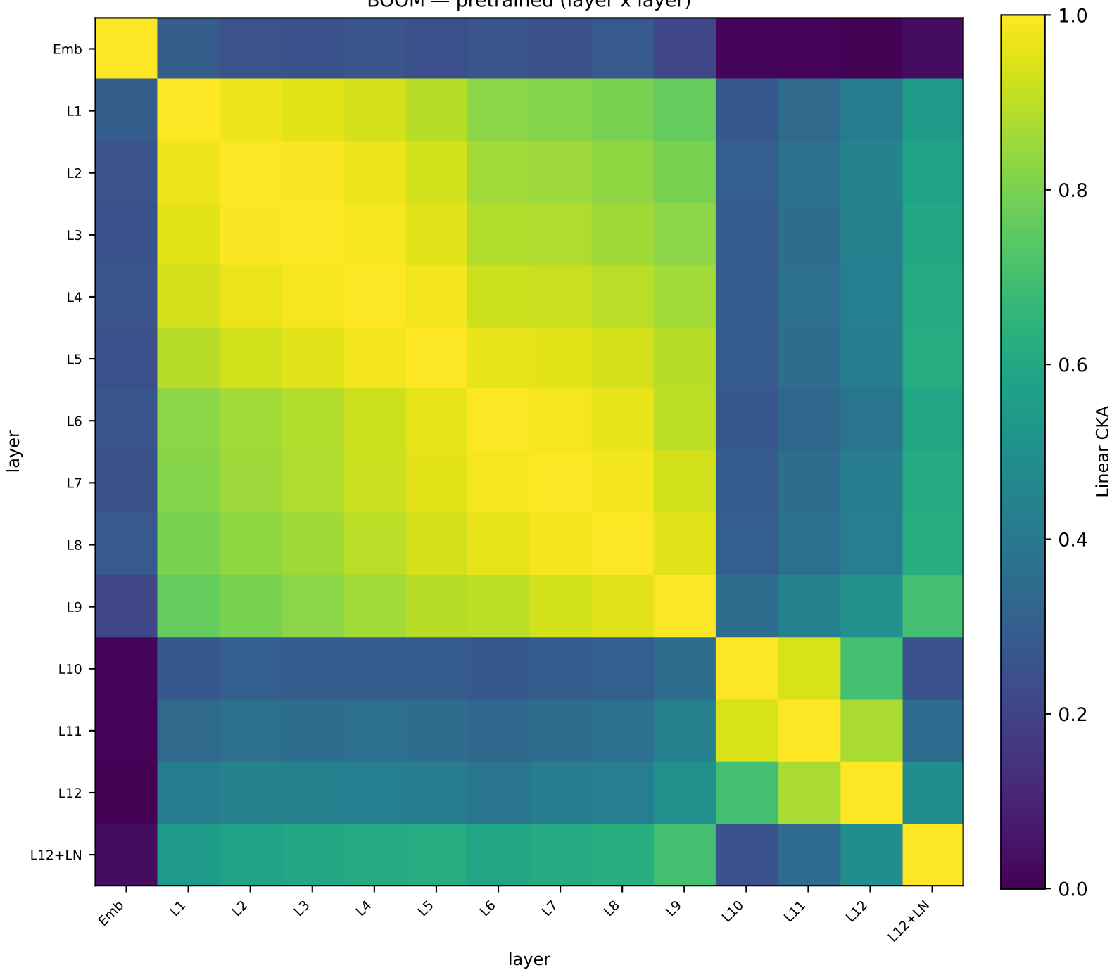
BOOM — pretrained (layer x layer)
