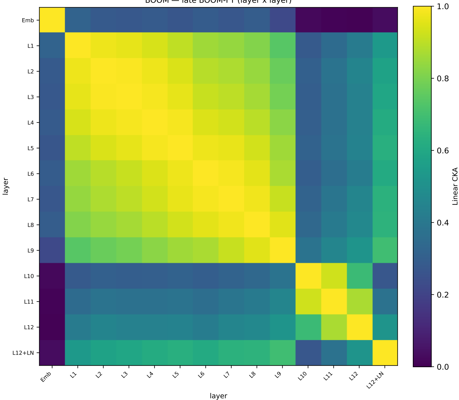
BOOM — late BOOM-FT (layer x layer)
