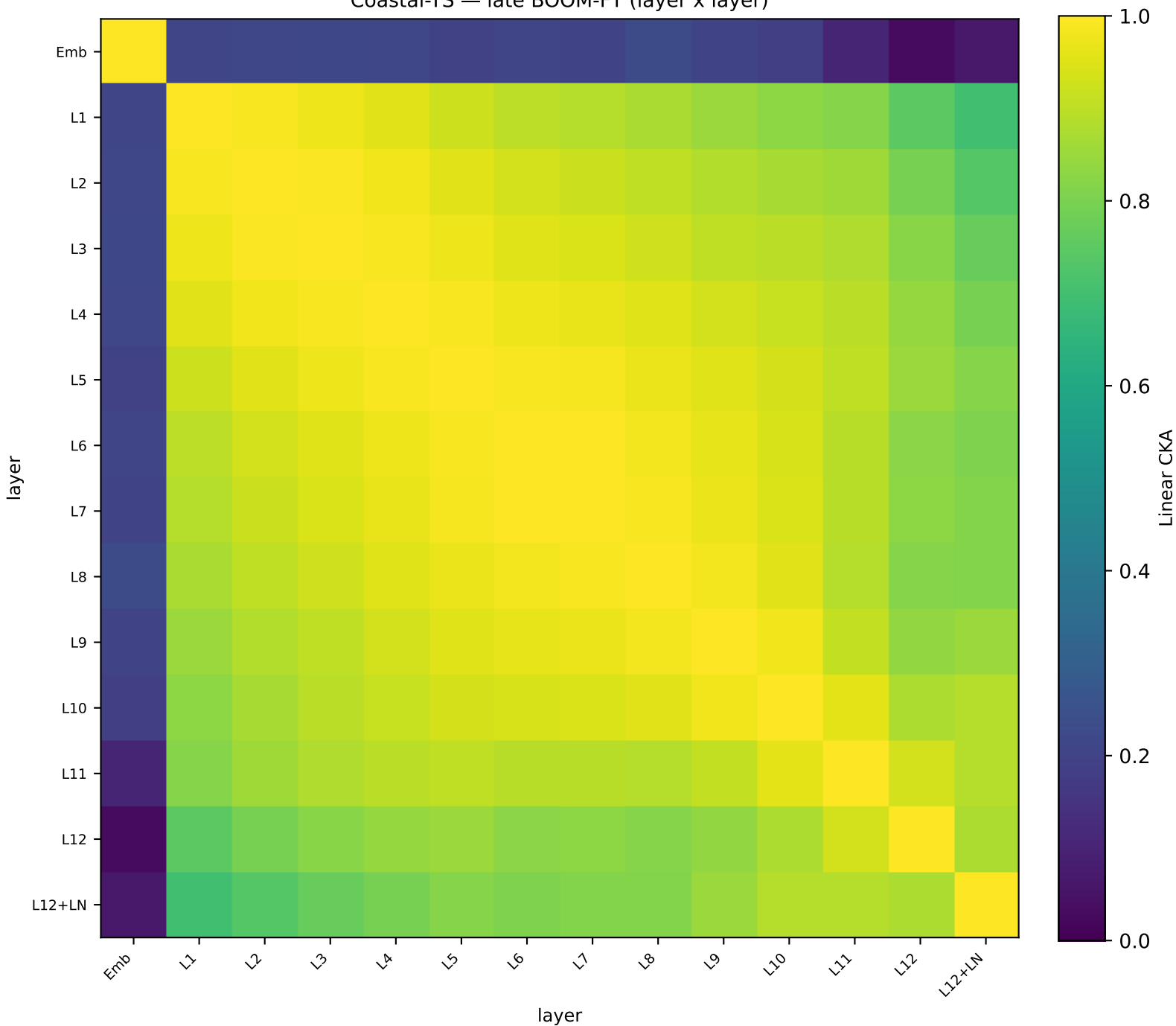
Coastal-TS — late BOOM-FT (layer x layer)
