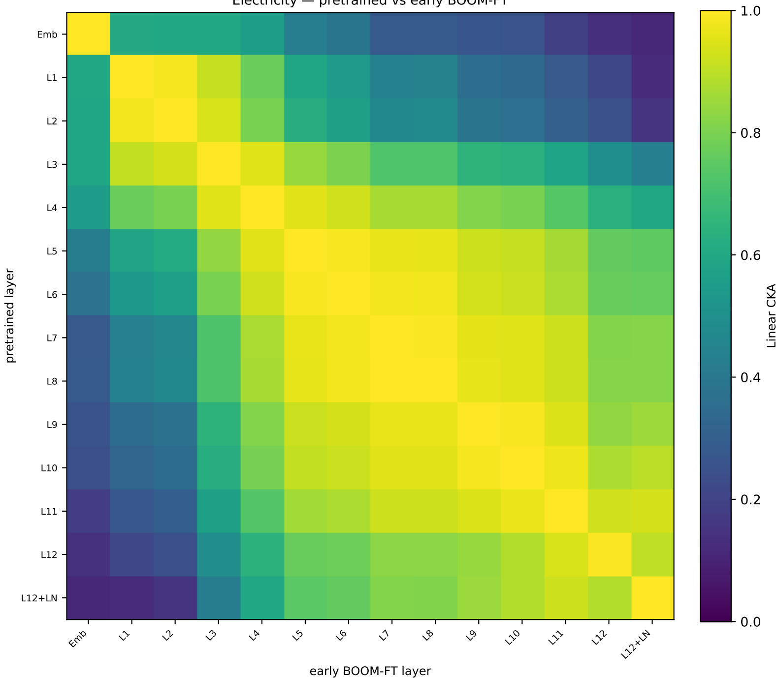
Electricity — pretrained vs early BOOM-FT
