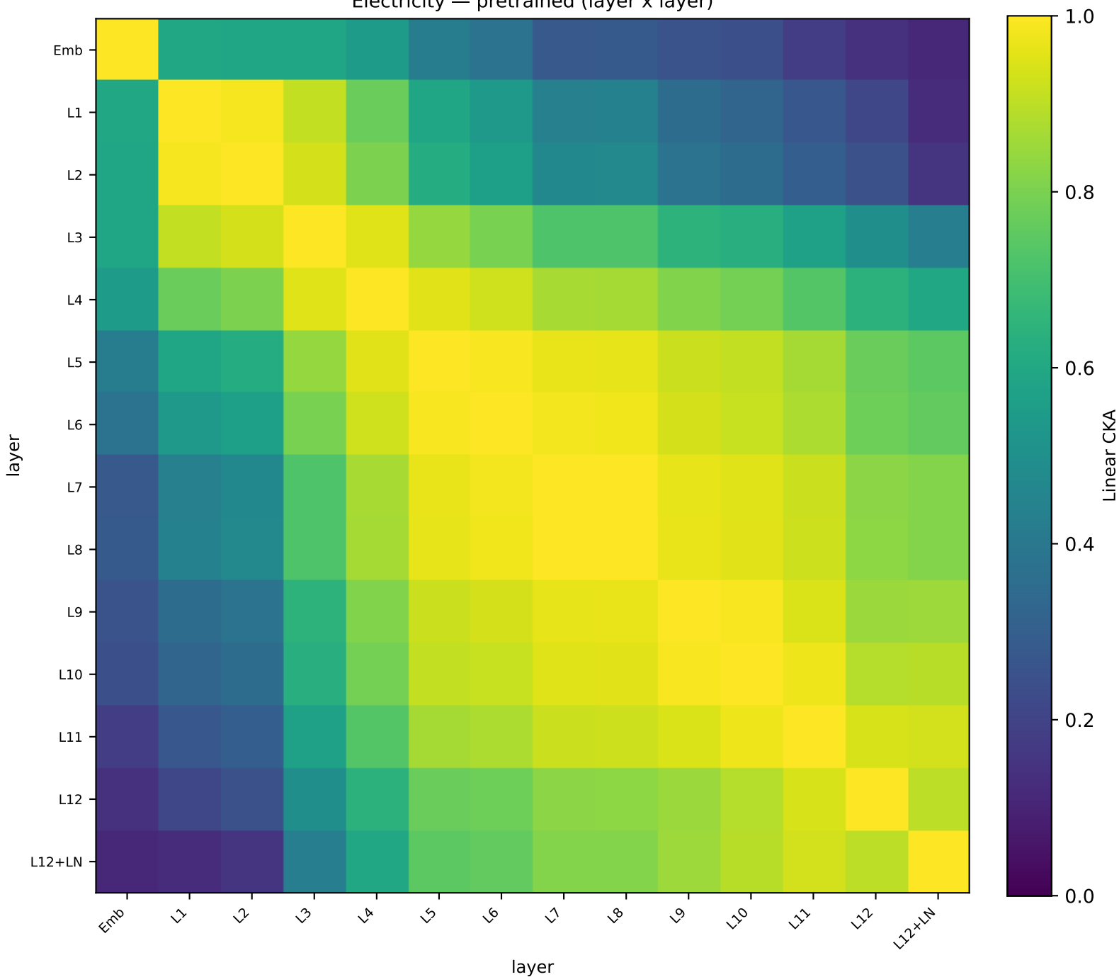
Electricity — pretrained (layer x layer)
