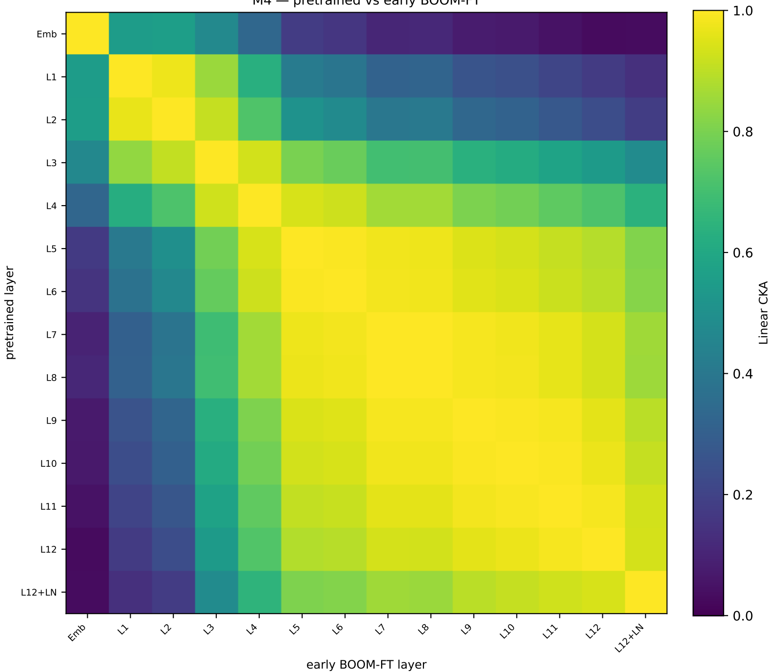
M4 — pretrained vs early BOOM-FT
