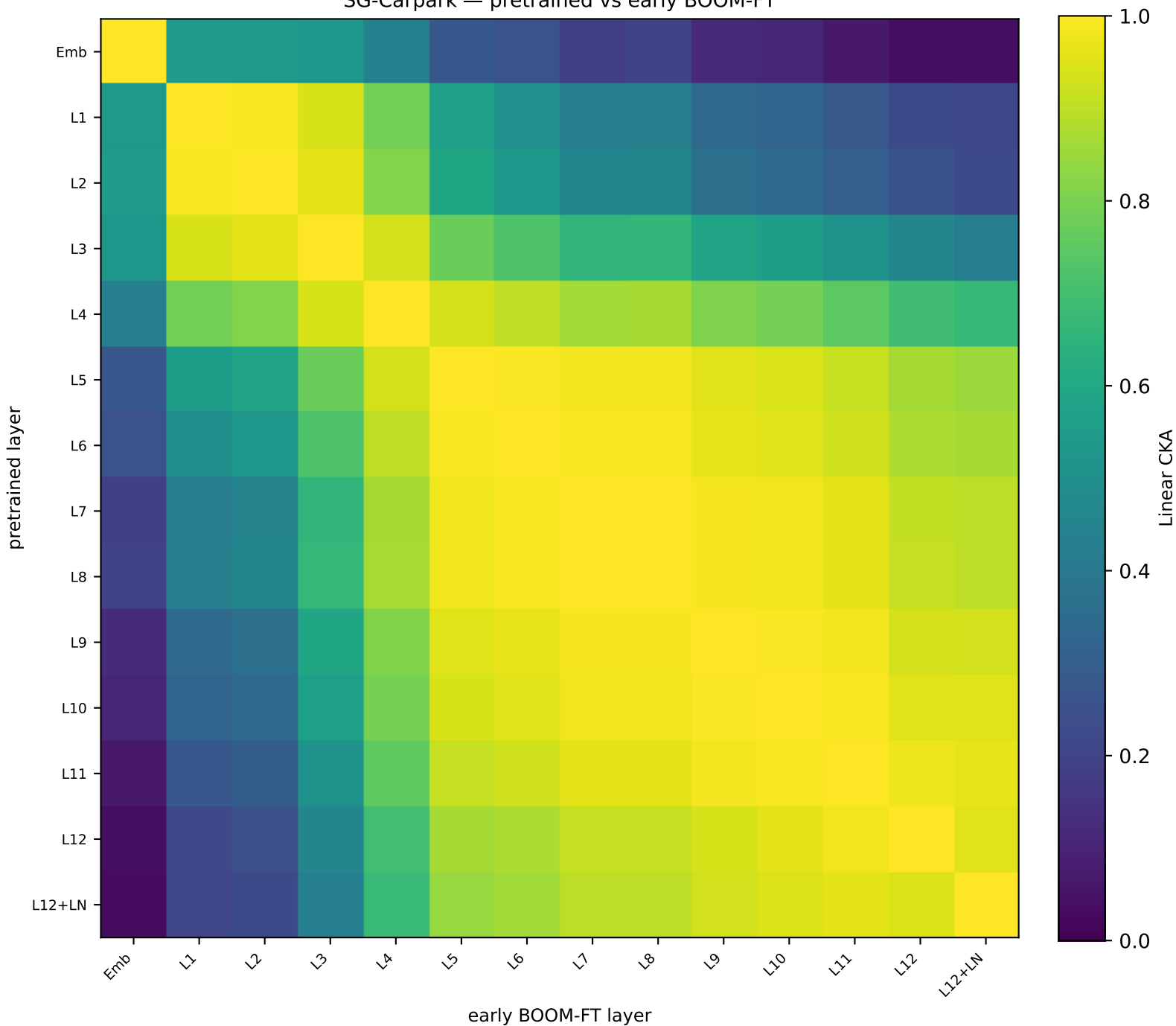
SG-Carpark — pretrained vs early BOOM-FT
