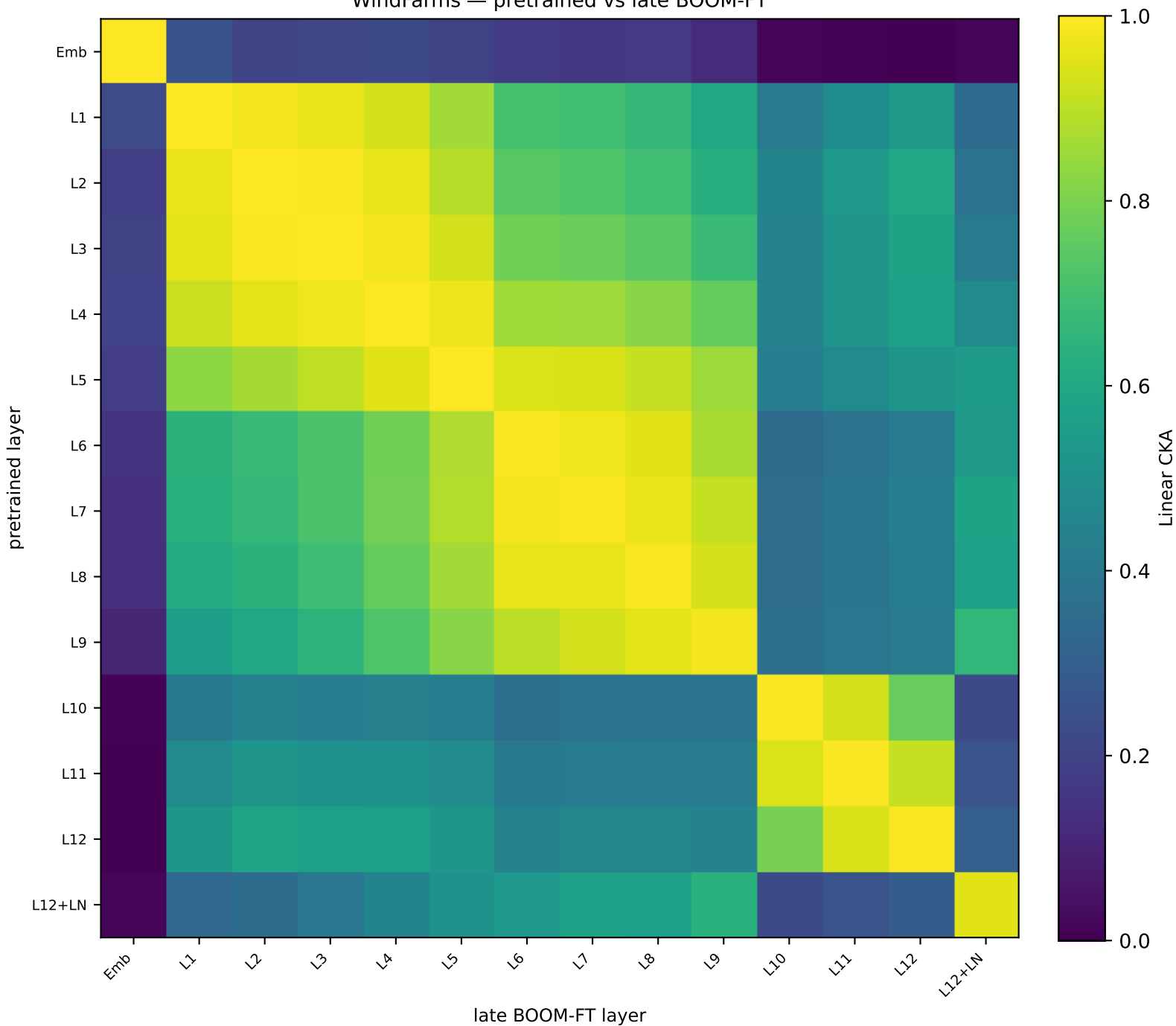
WindFarms — pretrained vs late BOOM-FT
