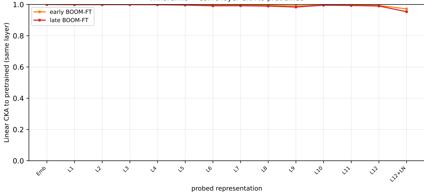
WindFarms — same-layer CKA to pretrained
