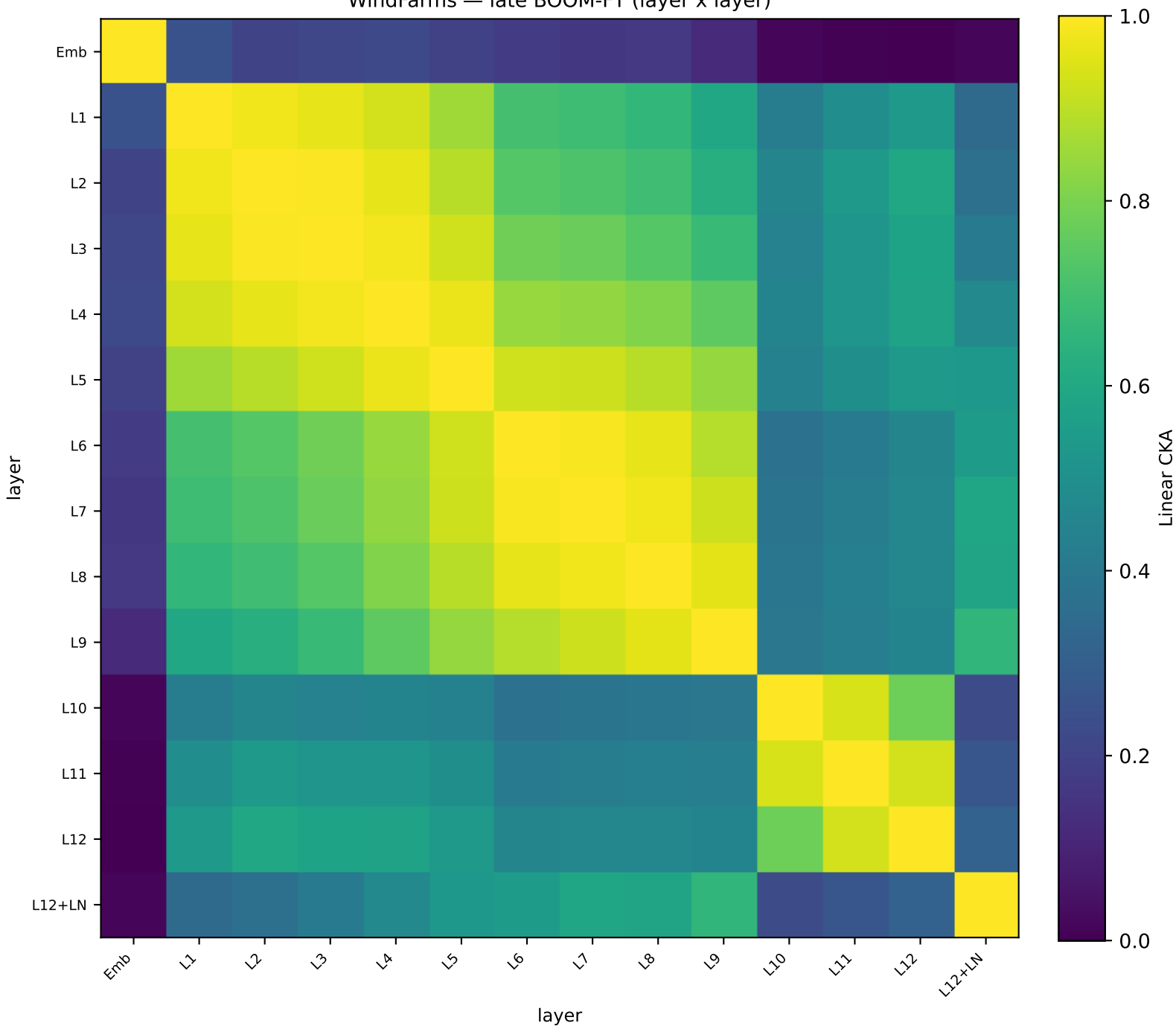
WindFarms — late BOOM-FT (layer x layer)
