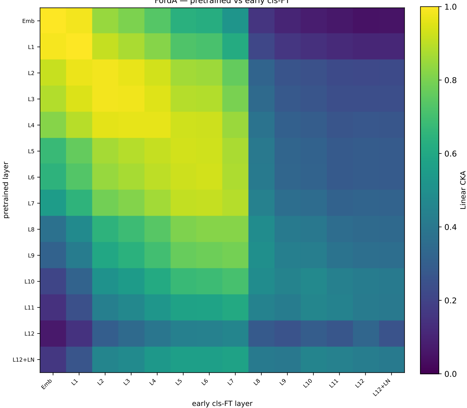
FordA — pretrained vs early cls-FT
