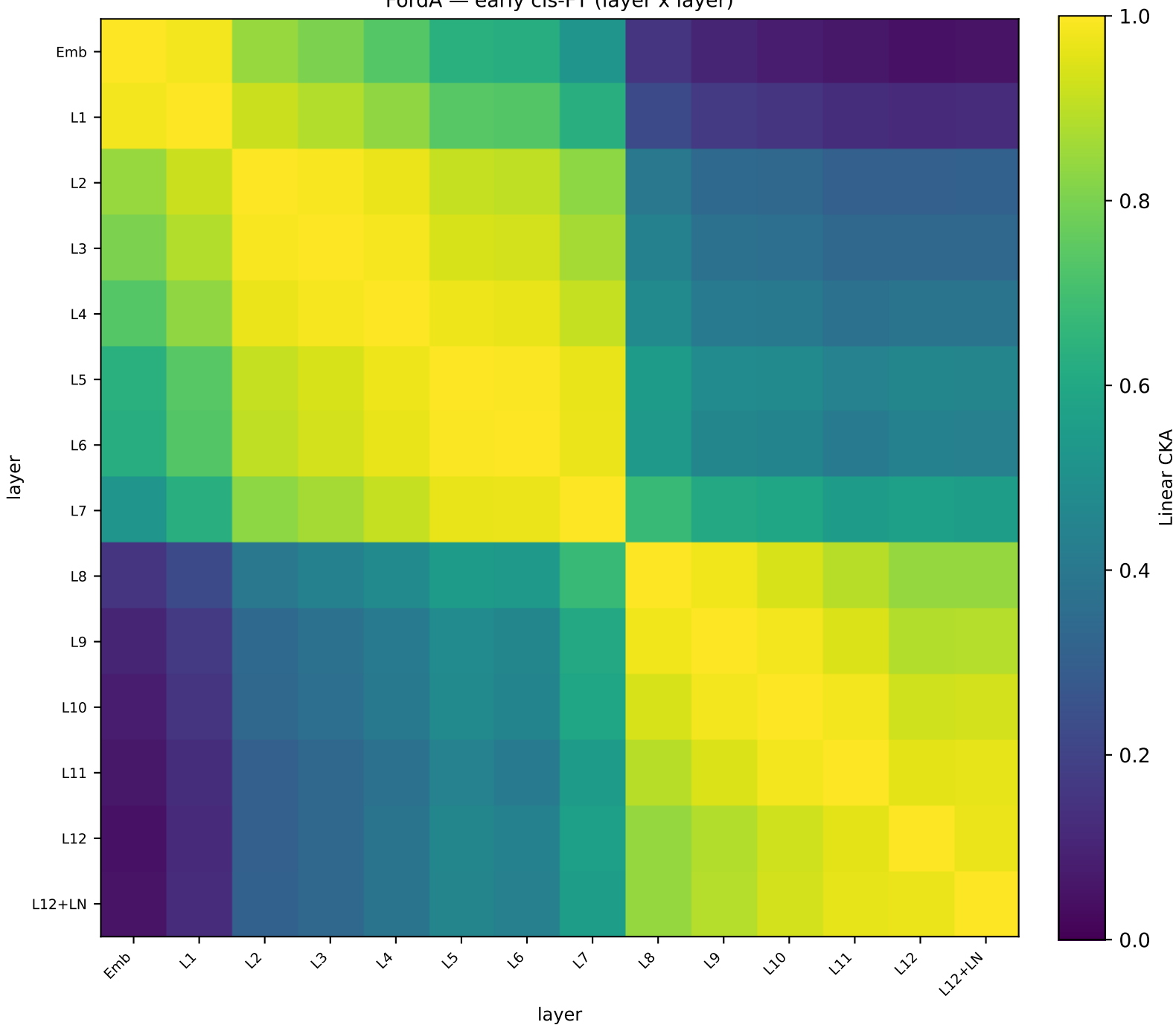
FordA — early cls-FT (layer x layer)
