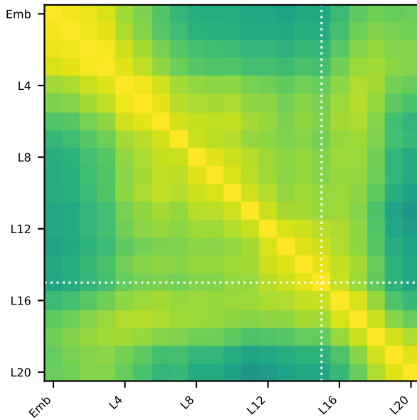
SG Carpark (PT-OOD, N=354) floor 0.782
