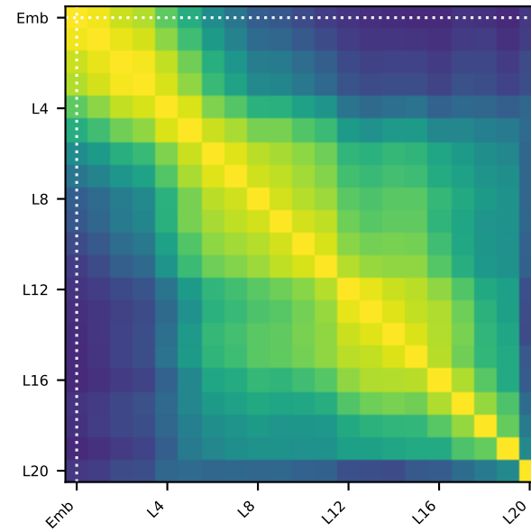
BOOM (PT-OOD, N=354) floor 0.782
