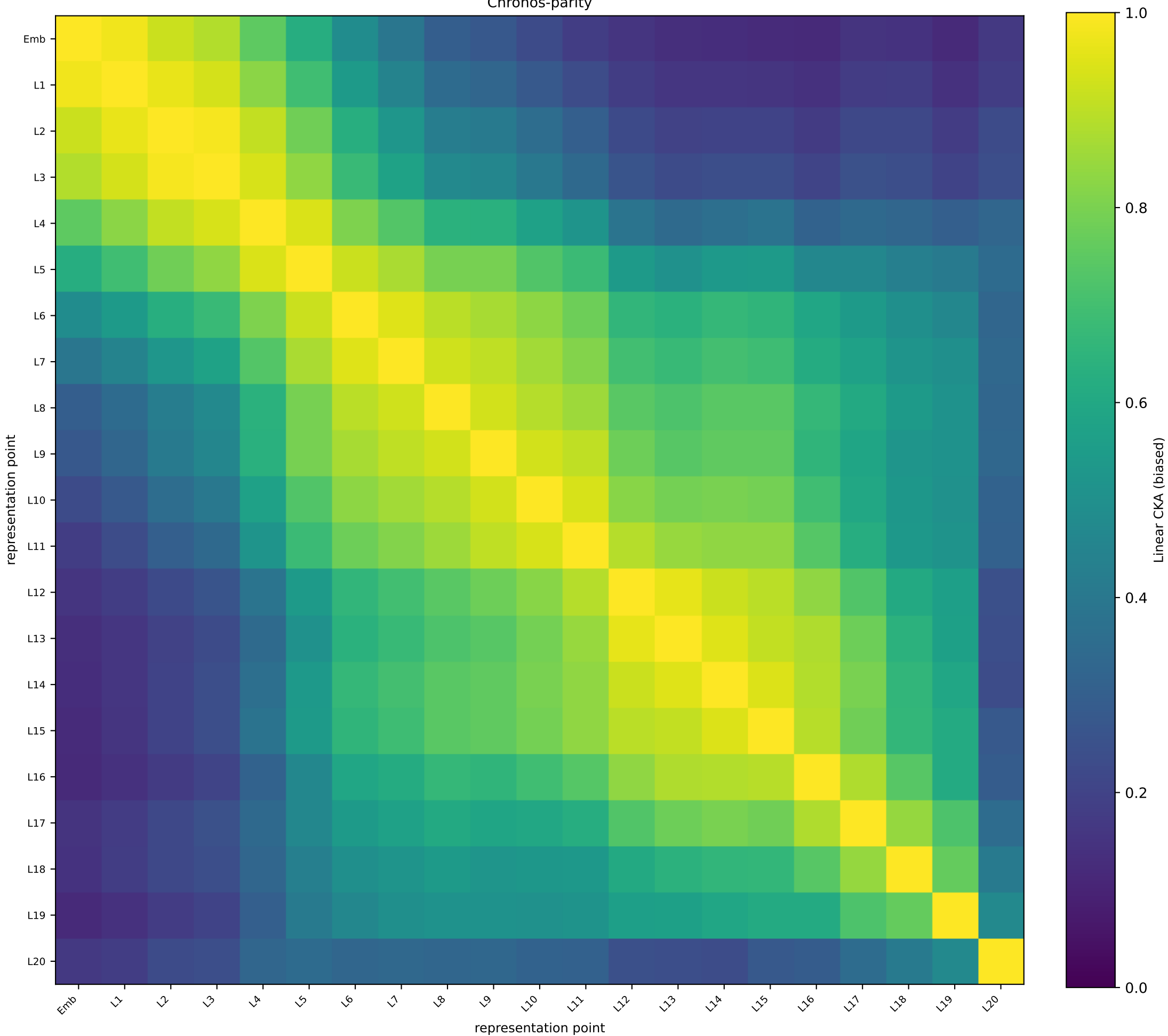
TimesFM-3 BOOM (PT-OOD) — token 15 biased linear CKA | test split | N=354 | independent-representation floor 0.782 Chronos-parity
