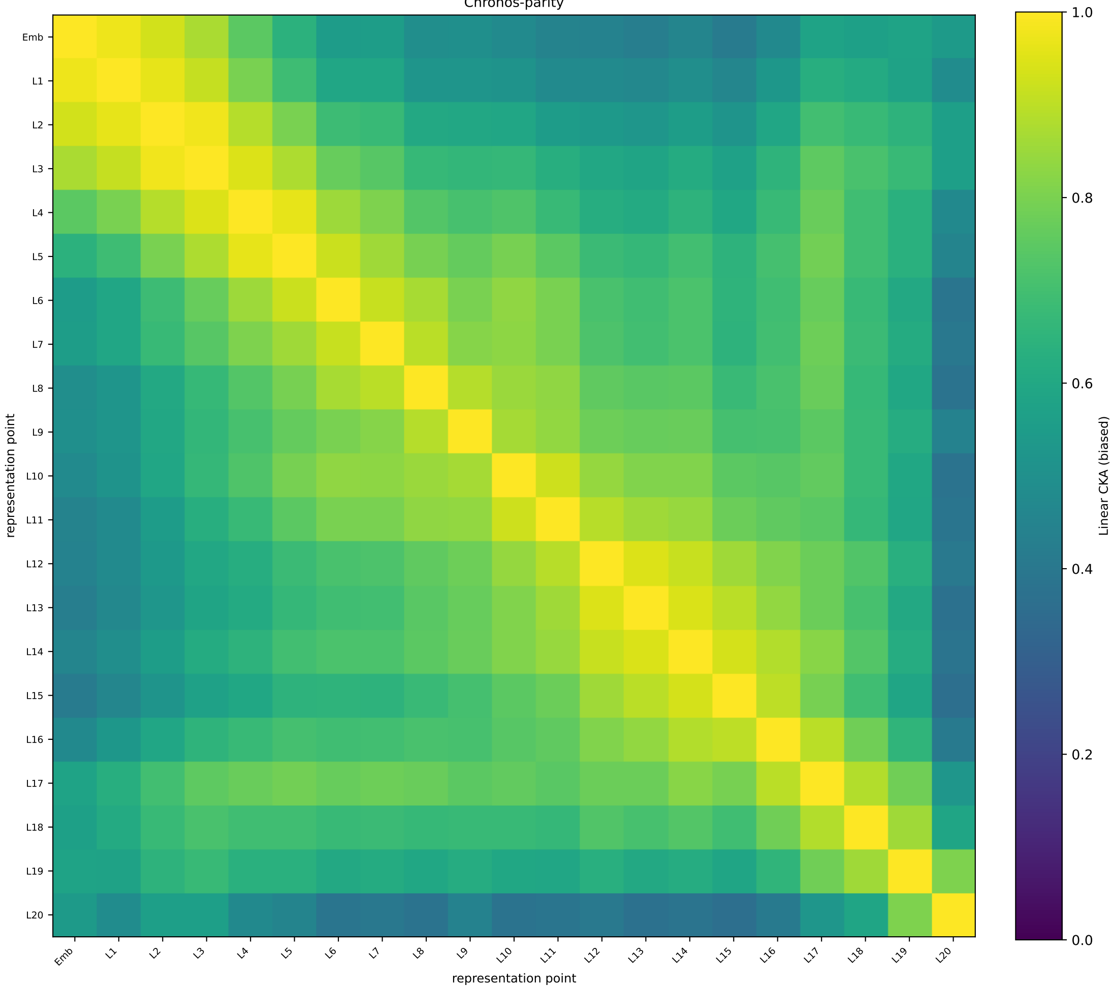
TimesFM-3 Coastal T-S (PT-OOD) — token 15 biased linear CKA | test split | N=48 | independent-representation floor 0.965 Chronos-parity
