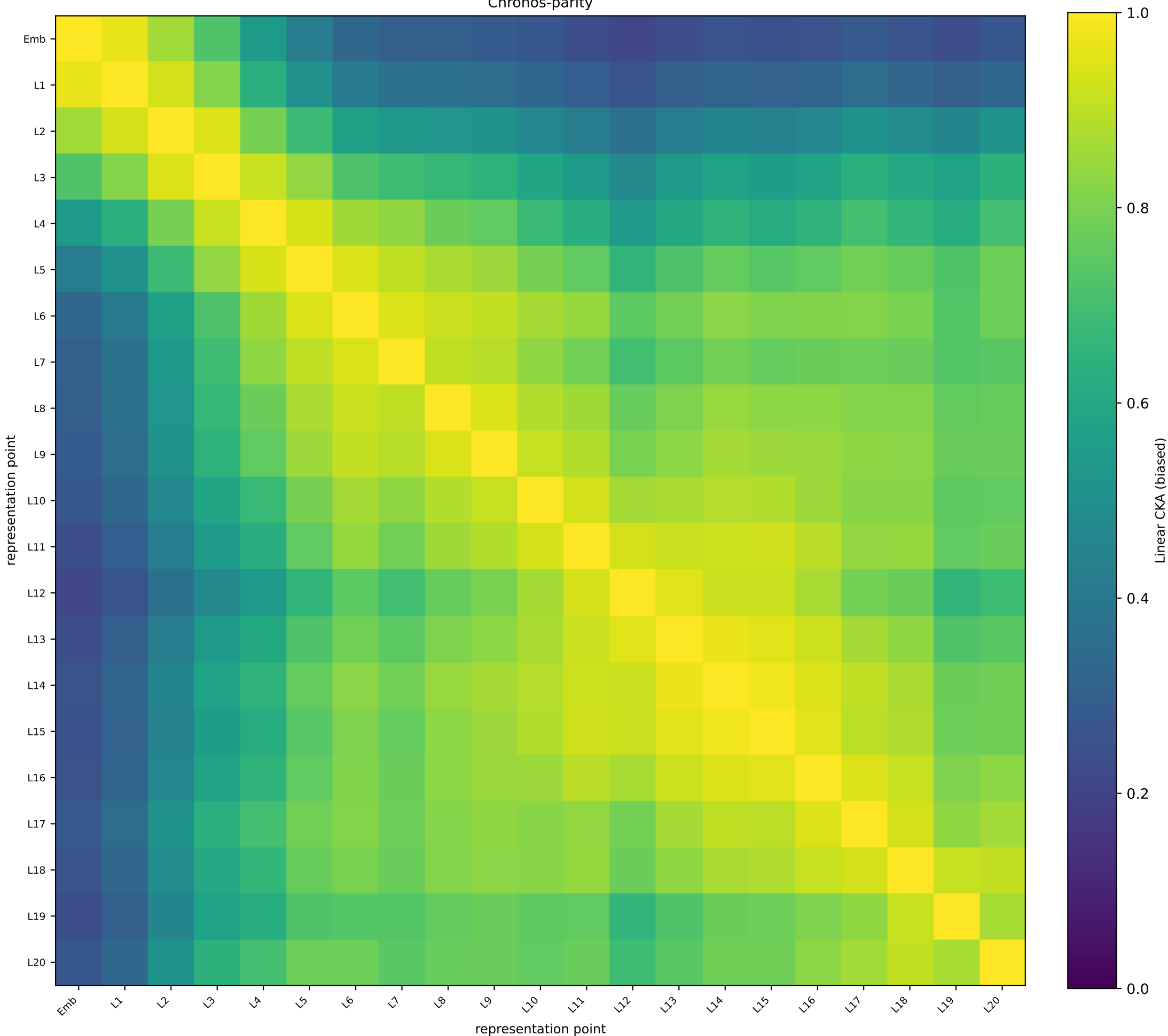
TimesFM-3 Uber TLC (PT-ID) — token 15 biased linear CKA | test split | N=262 | independent-representation floor 0.830 Chronos-parity
