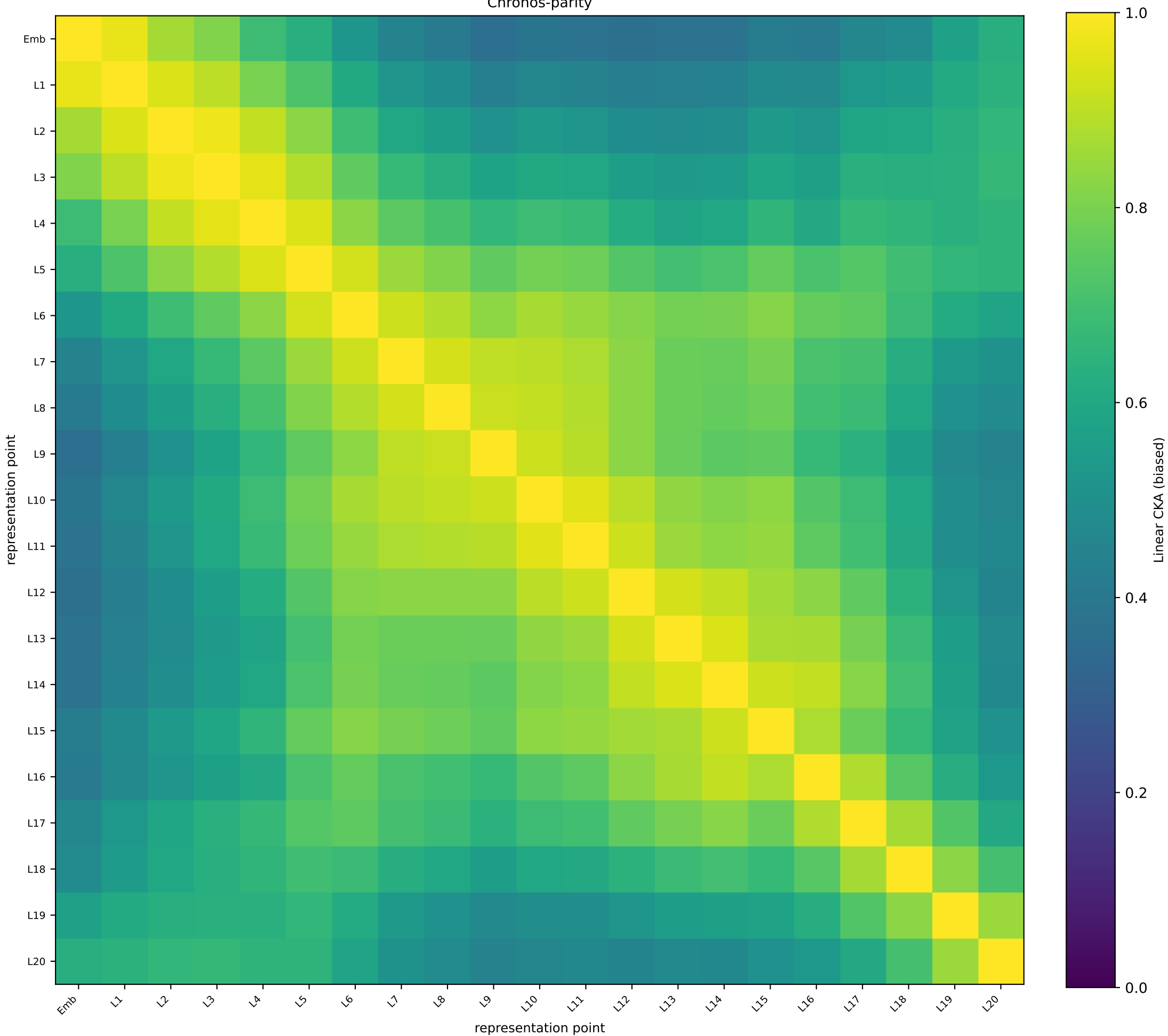
TimesFM-3 Wind Farms (PT-ID) — token 15 biased linear CKA | test split | N=262 | independent-representation floor 0.830 Chronos-parity
