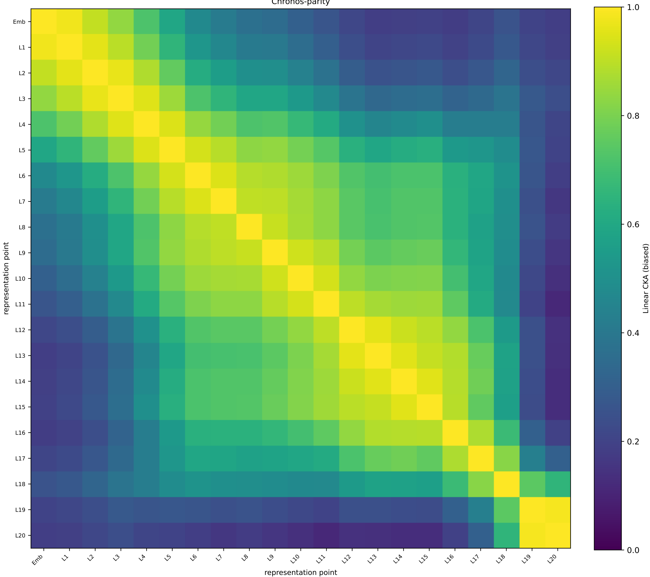
TimesFM-3 BOOM (PT-OOD) — token 15 biased linear CKA | train split | N=1394 | independent-representation floor 0.479 Chronos-parity
