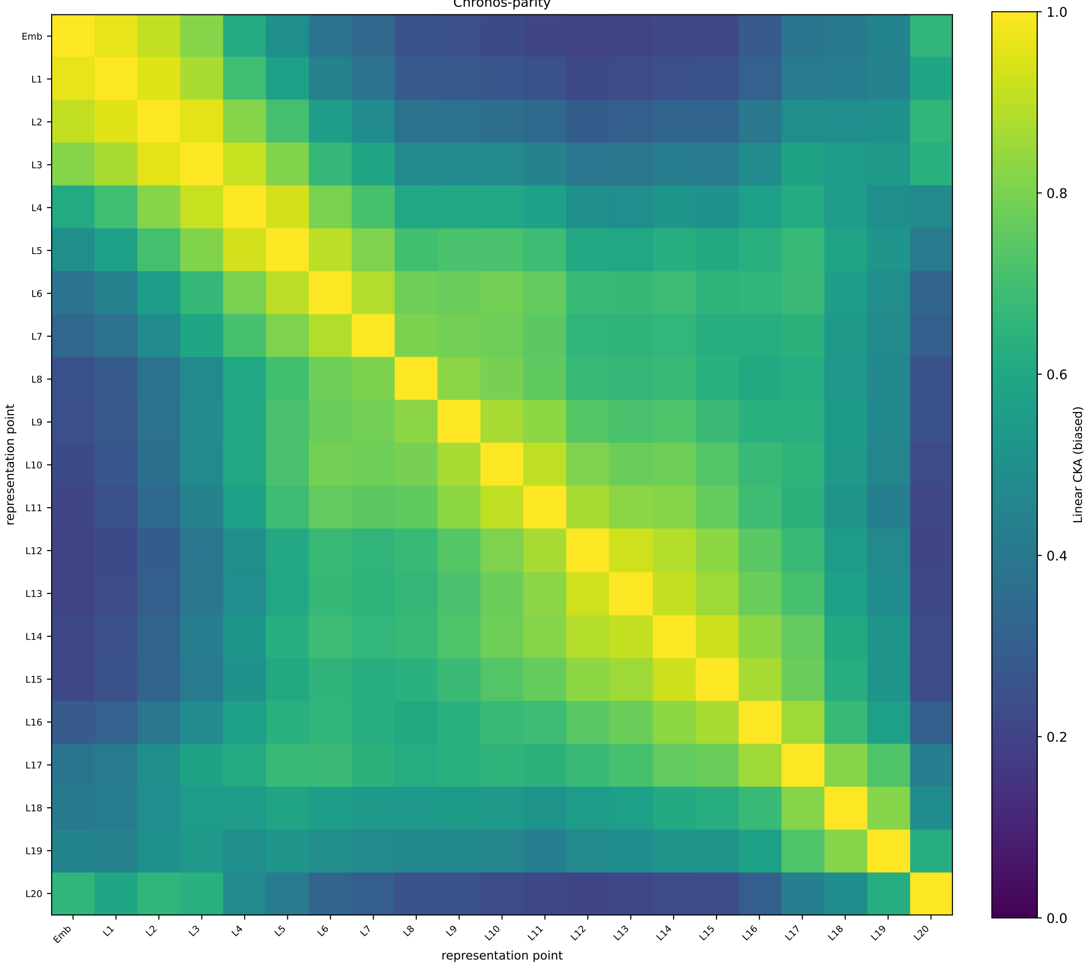
TimesFM-3 Coastal T-S (PT-OOD) — token 15 biased linear CKA | train split | N=1394 | independent-representation floor 0.479 Chronos-parity
