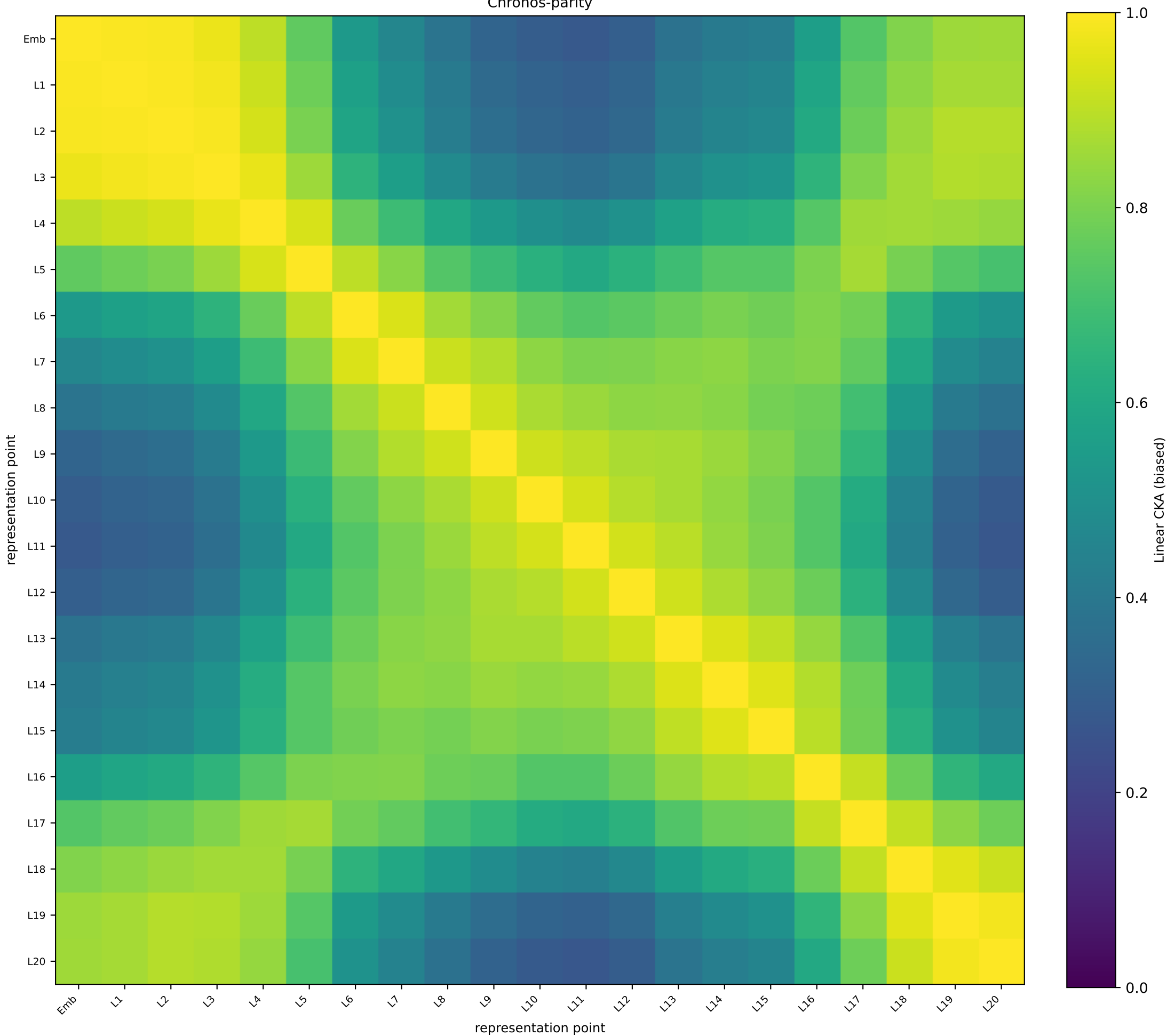
TimesFM-3 SG Carpark (PT-OOD) — token 15 biased linear CKA | train split | N=1394 | independent-representation floor 0.479 Chronos-parity
