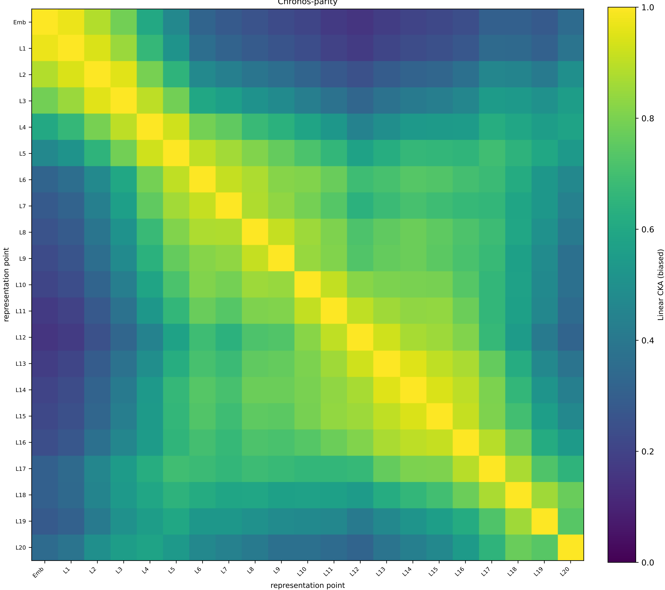
TimesFM-3 Uber TLC (PT-ID) — token 15 biased linear CKA | train split | N=1394 | independent-representation floor 0.479 Chronos-parity
