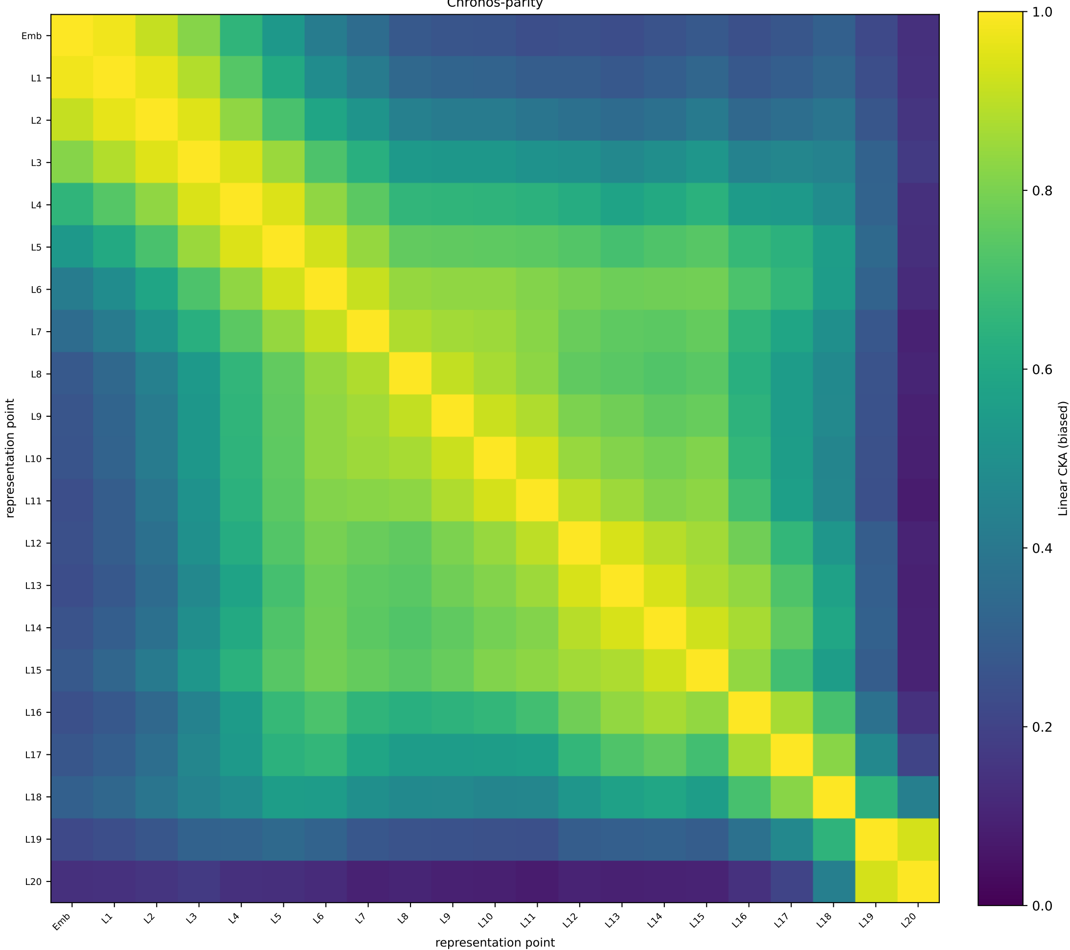
TimesFM-3 Wind Farms (PT-ID) — token 15 biased linear CKA | train split | N=1394 | independent-representation floor 0.479 Chronos-parity
