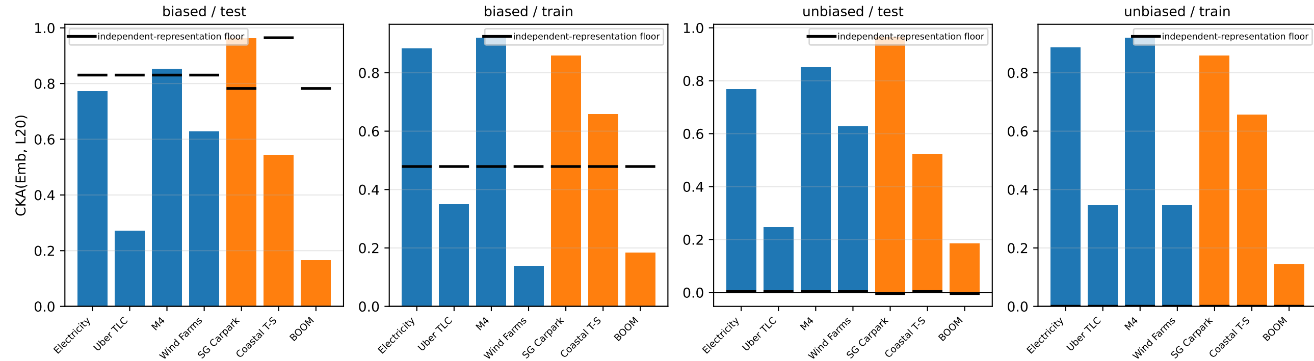
CKA(Emb, L20) against each estimator's own finite-sample floor biased sits near its floor at small N; unbiased is floor-free
