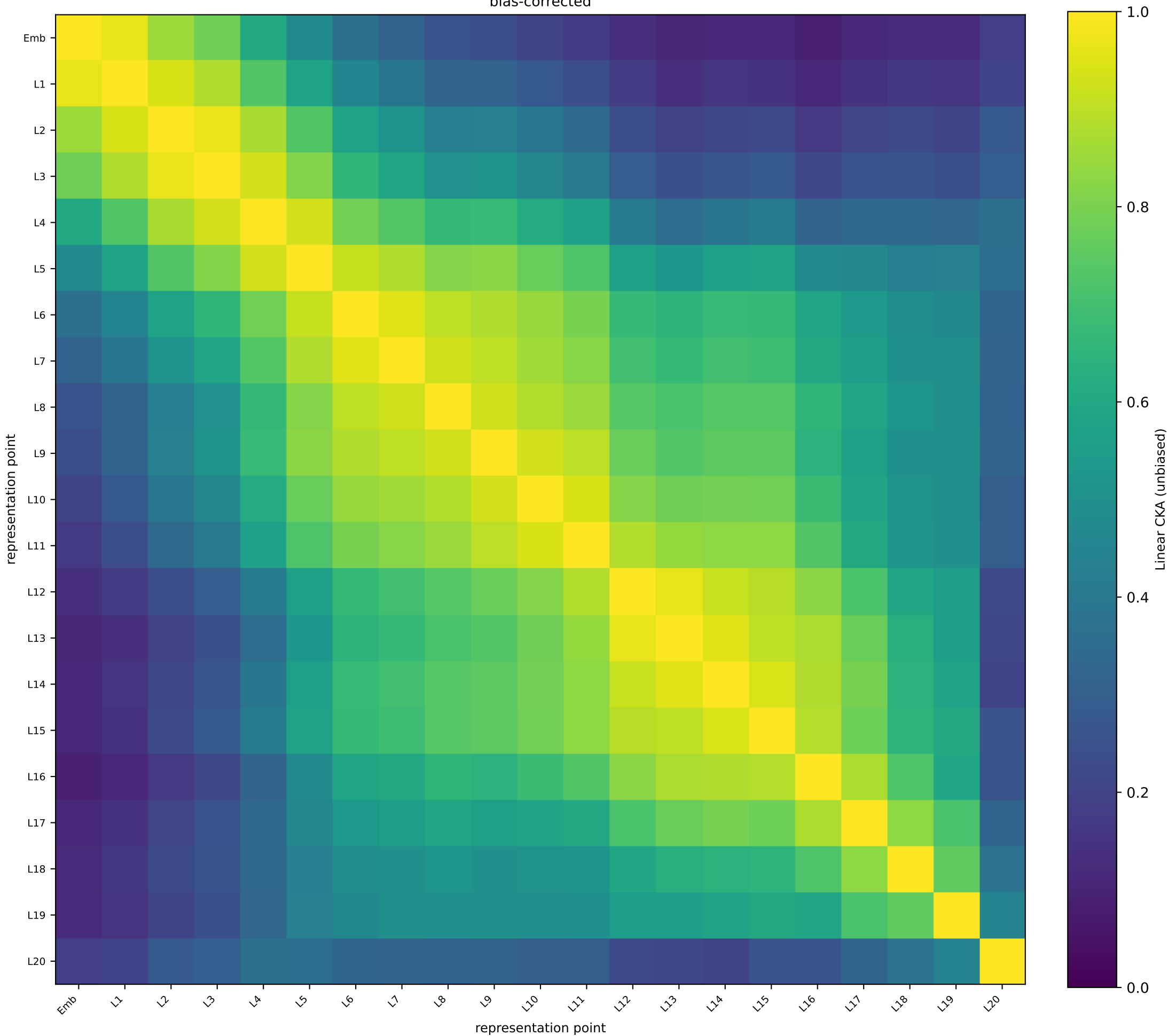
TimesFM-3 BOOM (PT-OOD) — token 15 unbiased linear CKA | test split | N=354 | independent-representation floor -0.004 bias-corrected
