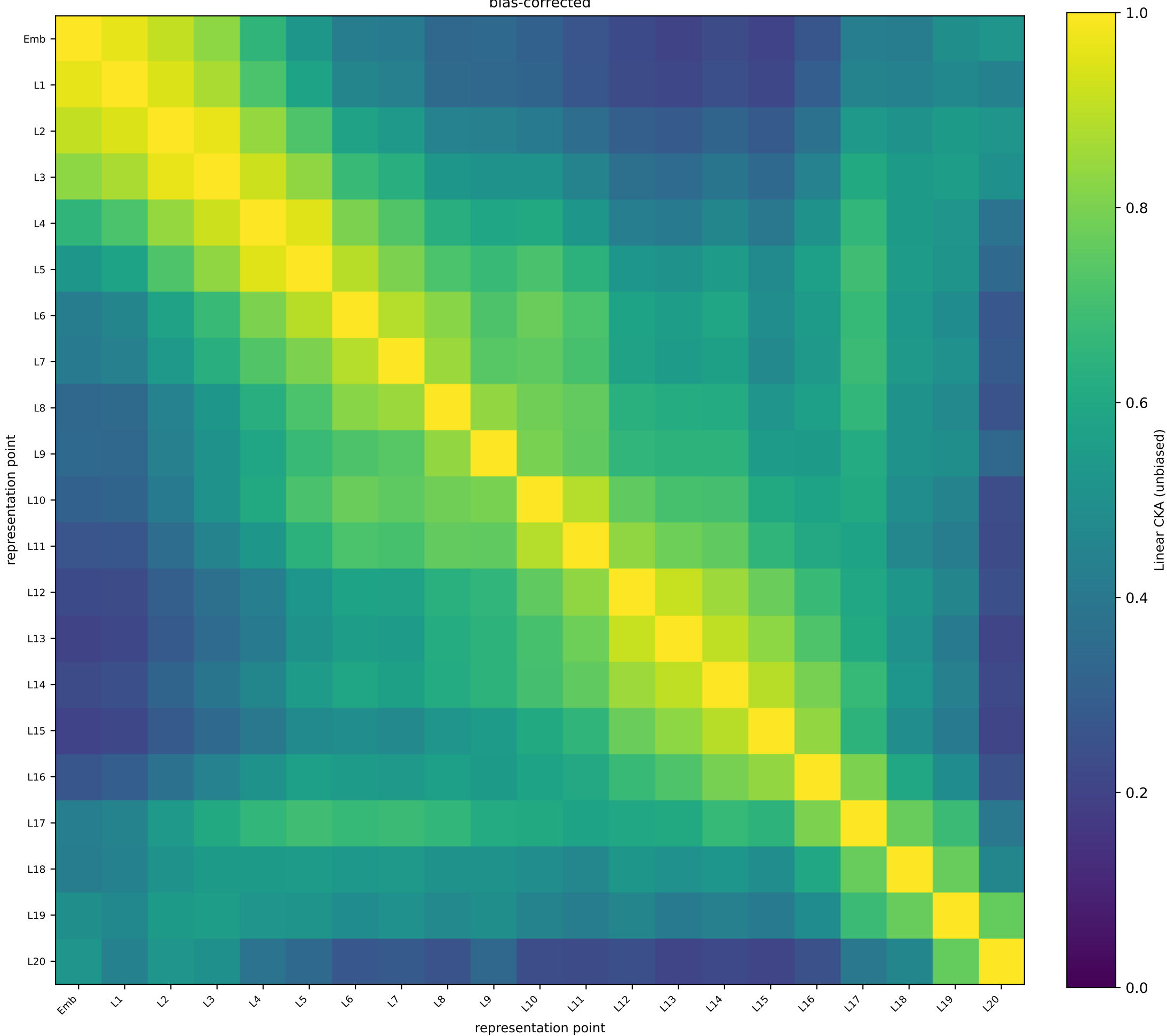
TimesFM-3 Coastal T-S (PT-OOD) — token 15 unbiased linear CKA | test split | N=48 | independent-representation floor 0.003 bias-corrected
