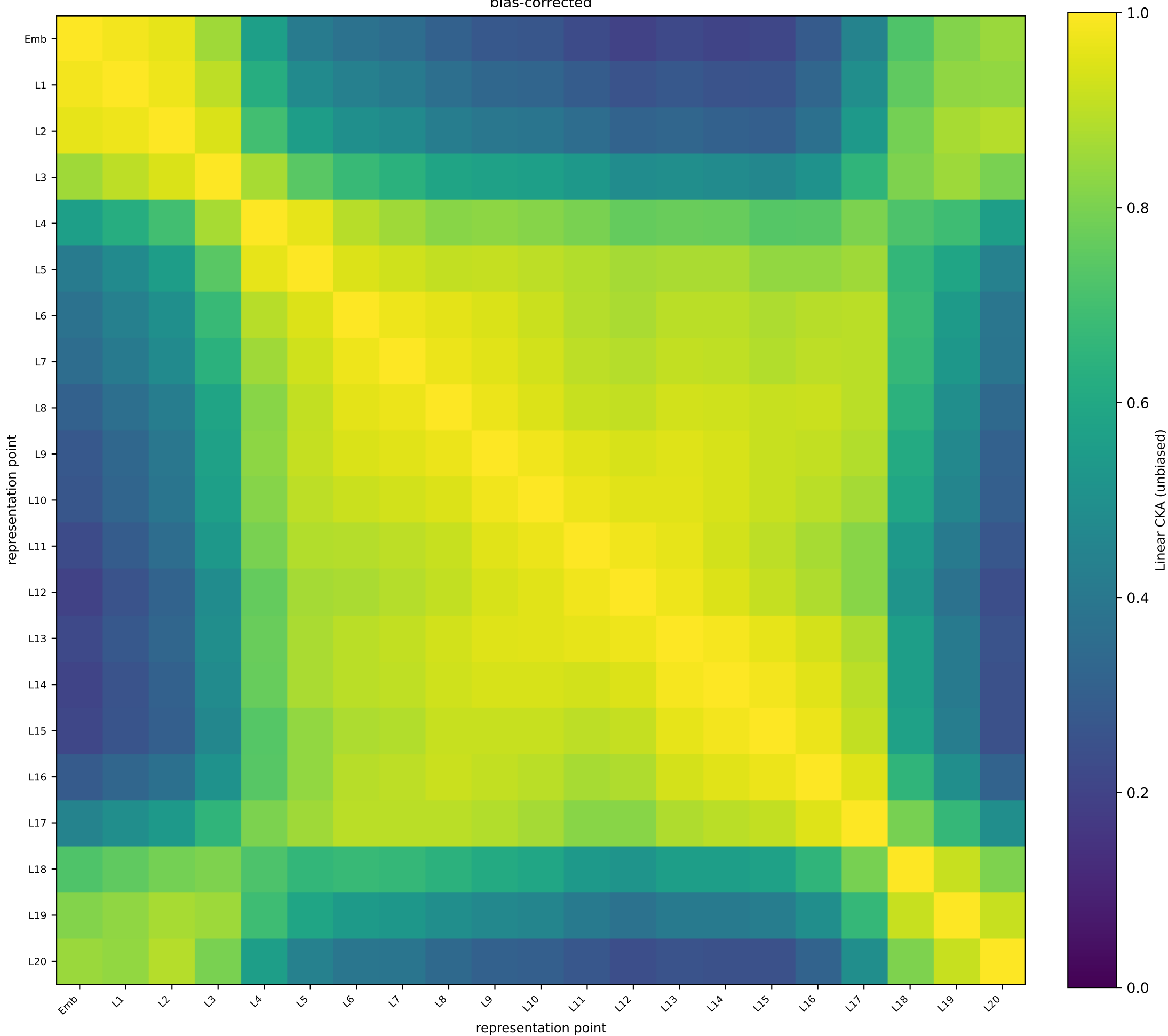
TimesFM-3 M4 (PT-ID) — token 15 unbiased linear CKA | test split | N=262 | independent-representation floor 0.003 bias-corrected
