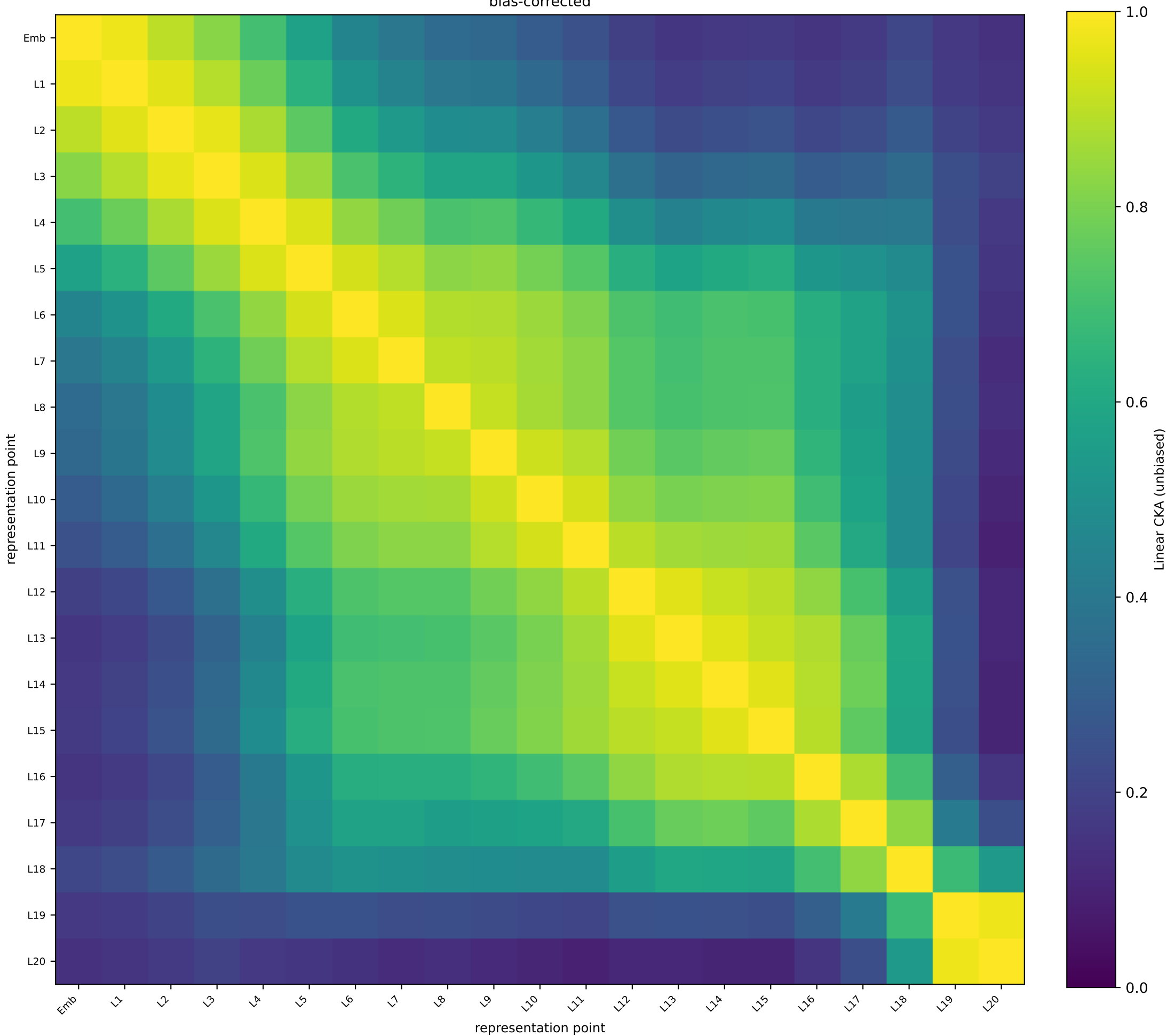
TimesFM-3 BOOM (PT-OOD) — token 15 unbiased linear CKA | train split | N=1394 | independent-representation floor 0.000 bias-corrected
