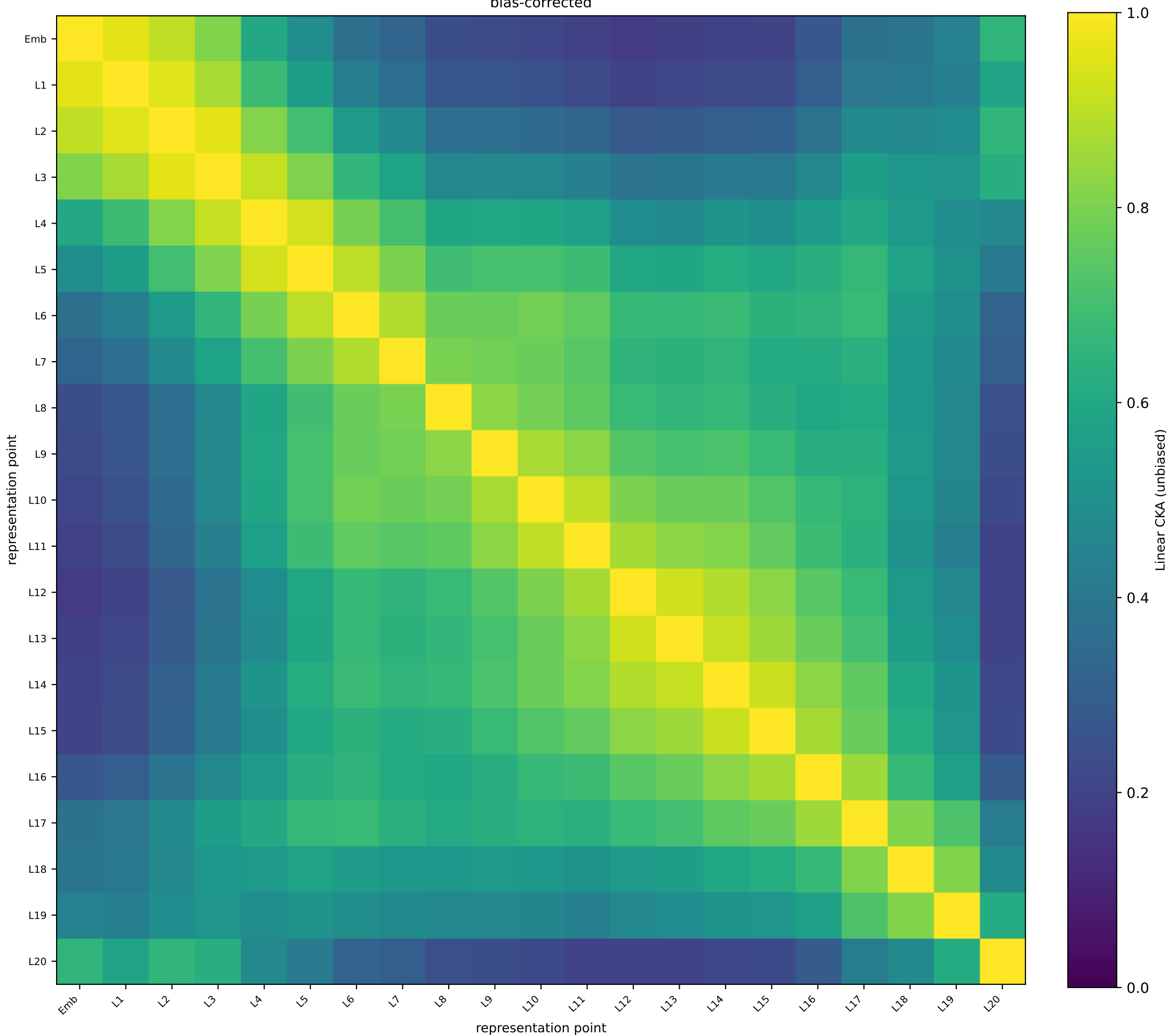
TimesFM-3 Coastal T-S (PT-OOD) — token 15 unbiased linear CKA | train split | N=1394 | independent-representation floor 0.000 bias-corrected
