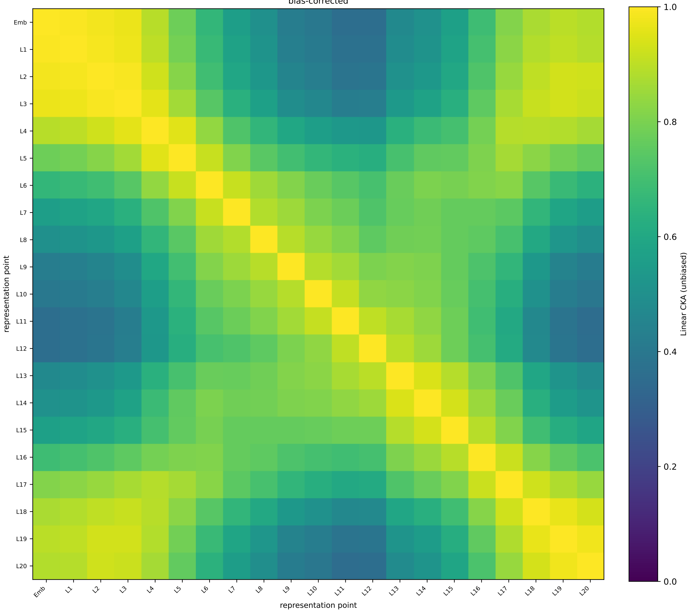
TimesFM-3 Electricity (PT-ID) — token 15 unbiased linear CKA | train split | N=1394 | independent-representation floor 0.000 bias-corrected
