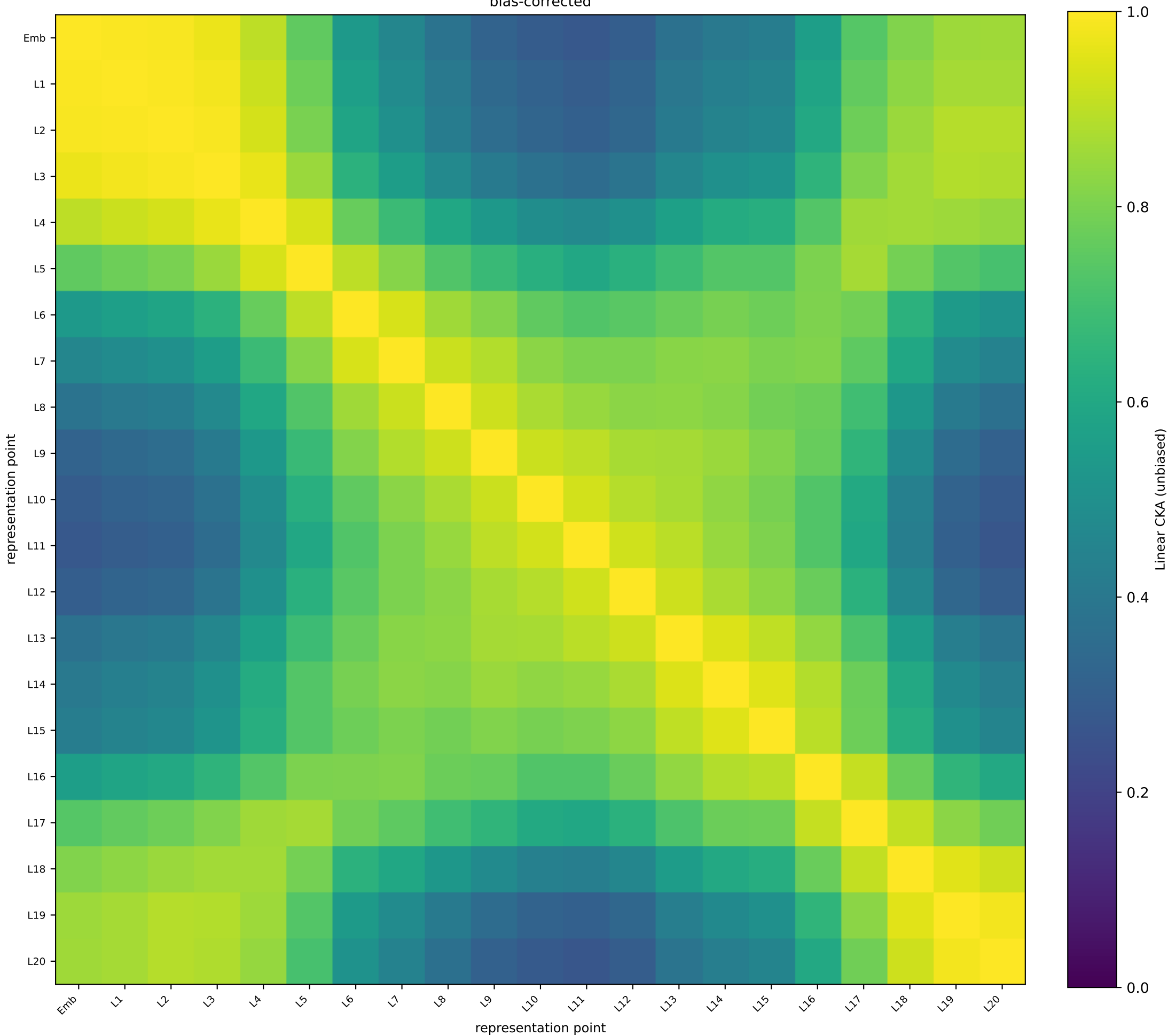
TimesFM-3 SG Carpark (PT-OOD) — token 15 unbiased linear CKA | train split | N=1394 | independent-representation floor 0.000 bias-corrected
